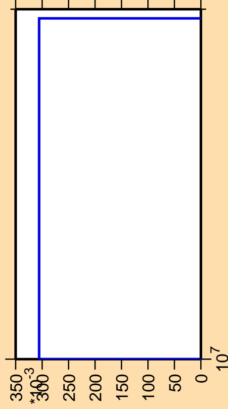
\Delta\sigma/\sigma vs. E for ^{110}\text{Pd}(n,\text{nd})
