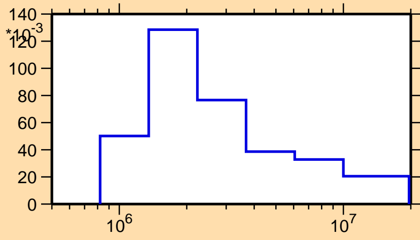
\sigma vs. E for ^{110}\text{Pd}(n,n_3)
