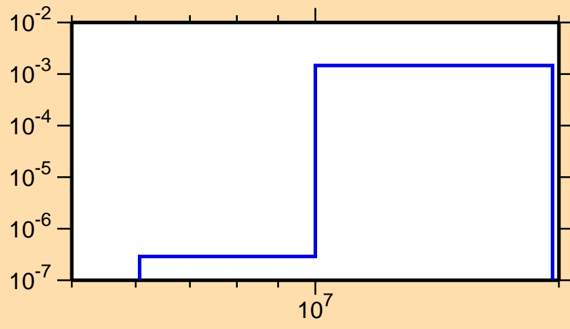
\sigma vs. E for ^{110}\text{Pd}(n,p)
