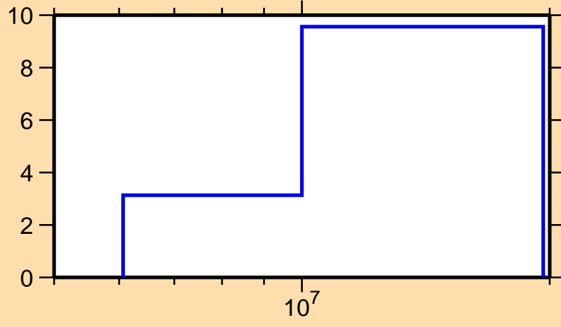
\Delta\sigma/\sigma vs. E for ^{110}\text{Pd}(n,n\text{cont.})
