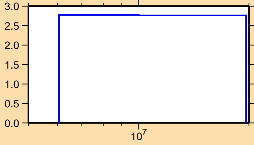
\Delta\sigma/\sigma vs. E for ^{110}\text{Pd}(n,el.)
