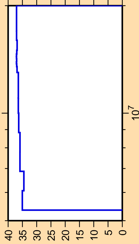
\Delta\sigma/\sigma vs. E for ^{111}\text{Pd}(n,\gamma)
