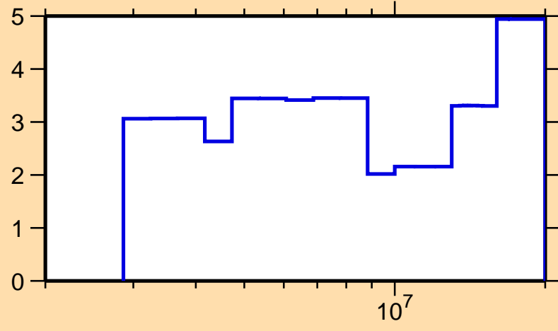
\Delta\sigma/\sigma vs. E for ^{111}\text{Pd}(n,\text{el.})
