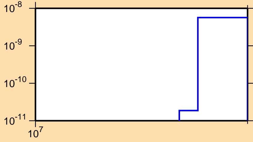
\sigma vs. E for ^{111}\text{Pd}(n,2n\alpha)
