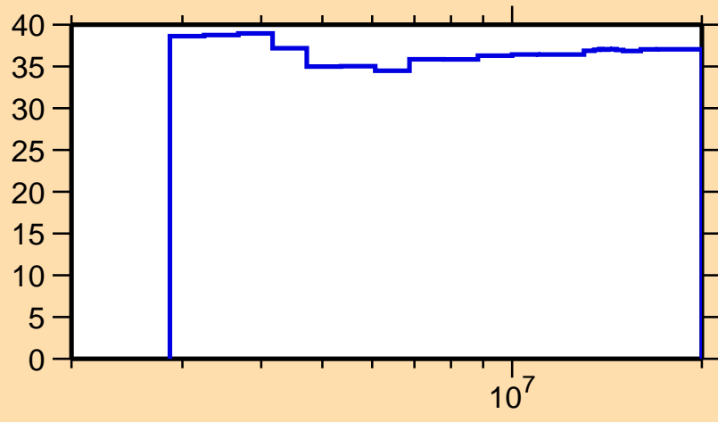
\Delta\sigma/\sigma vs. E for ^{111}\text{Pd}(n,\gamma)
