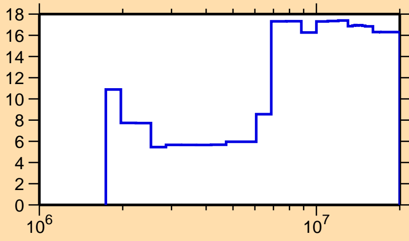
\Delta\sigma/\sigma vs. E for ^{111}\text{Pd}(n,n\text{cont.})
