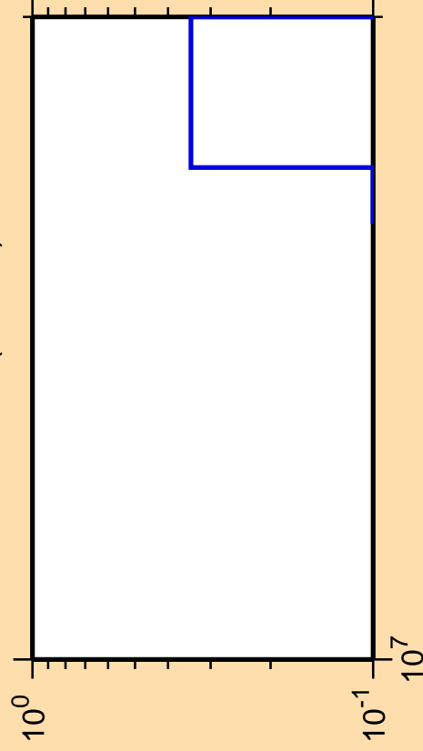
\Delta\sigma/\sigma vs. E for ^{111}\text{Pd}(n,\text{He3})
