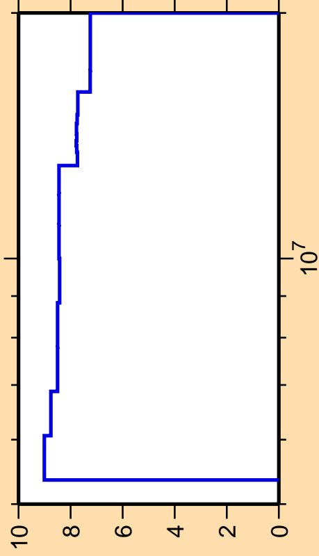
\Delta\sigma/\sigma vs. E for ^{111}\text{Pd}(n,n_1)
