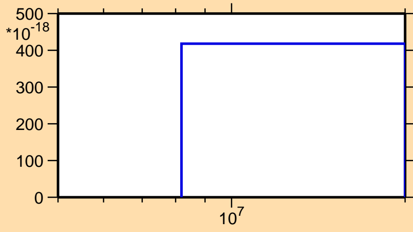
\sigma vs. E for ^{111}\text{Pd}(n,\text{He}3)
