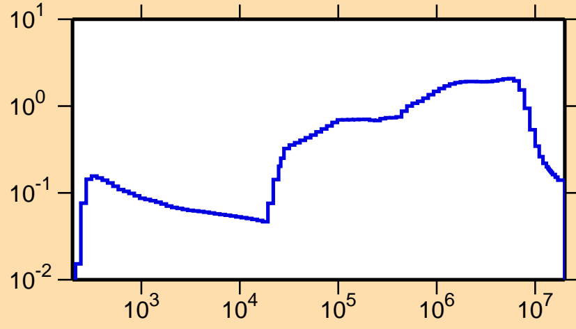
\sigma vs. E for ^{111}\text{Pd}(n,\text{inel.})
