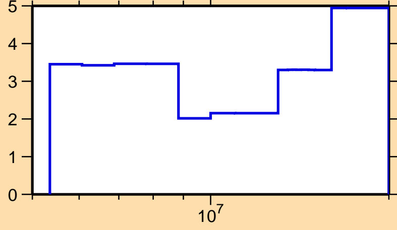
\Delta\sigma/\sigma vs. E for ^{111}\text{Pd}(n,\text{el.})
