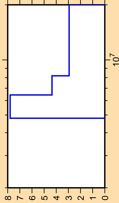
\Delta\sigma/\sigma vs. E for ^{111}\text{Pd}(n,2n)
