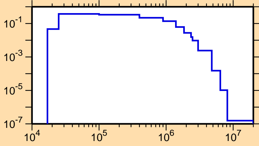
\sigma vs. E for ^{111}\text{Pd}(n,n_3)
