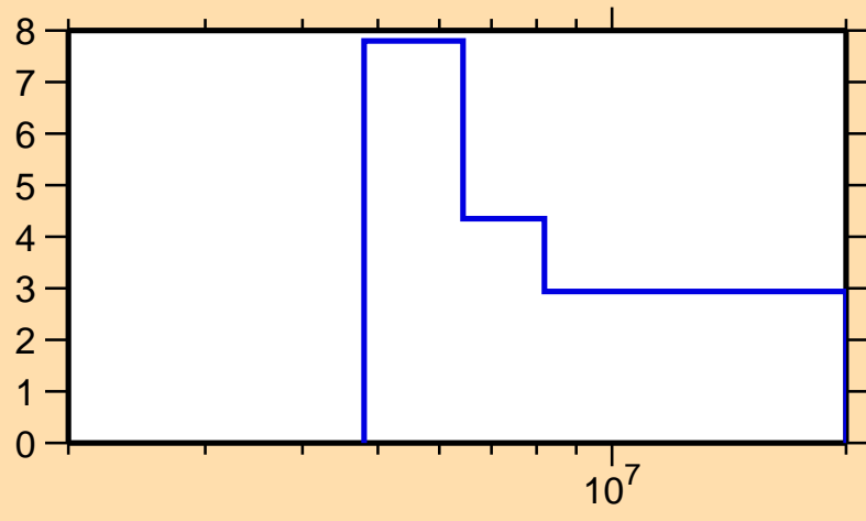
\Delta\sigma/\sigma vs. E for ^{111}\text{Pd}(n,2n)
