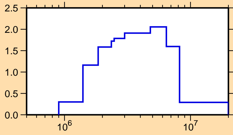
\sigma vs. E for ^{111}\text{Pd}(n,n\text{cont.})
