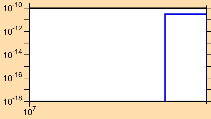
\sigma vs. E for ^{112}\text{Pd}(n,\text{nd})
