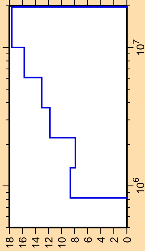
\Delta\sigma/\sigma vs. E for ^{112}\text{Pd}(n,n_3)
