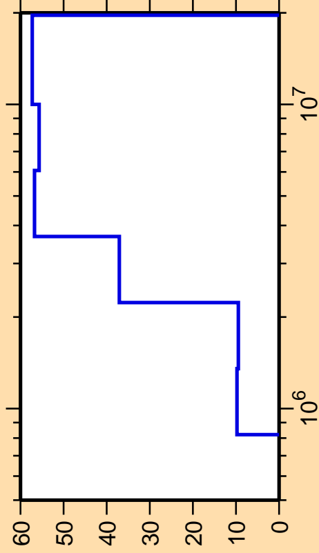
\Delta\sigma/\sigma vs. E for ^{112}\text{Pd}(n,n_4)
