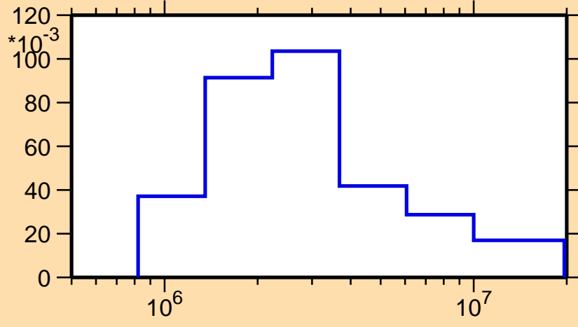
\sigma vs. E for ^{112}\text{Pd}(n,n_3)
