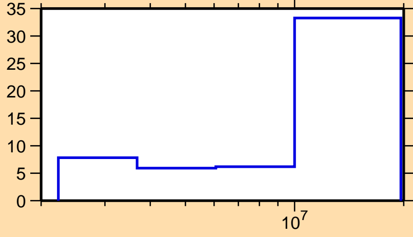
\Delta\sigma/\sigma vs. E for ^{112}\text{Pd}(n,n\text{cont.})
