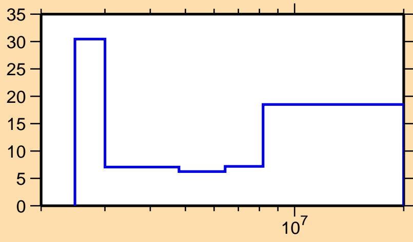
\Delta\sigma/\sigma vs. E for ^{112}\text{Pd}(n,n\text{cont.})
