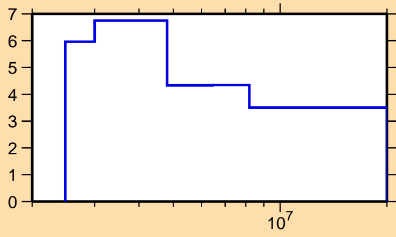
\Delta\sigma/\sigma vs. E for ^{112}\text{Pd}(n,\text{nonel.})
