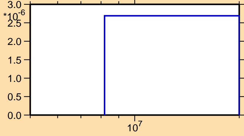
\sigma vs. E for ^{112}\text{Pd}(n,n\alpha)
