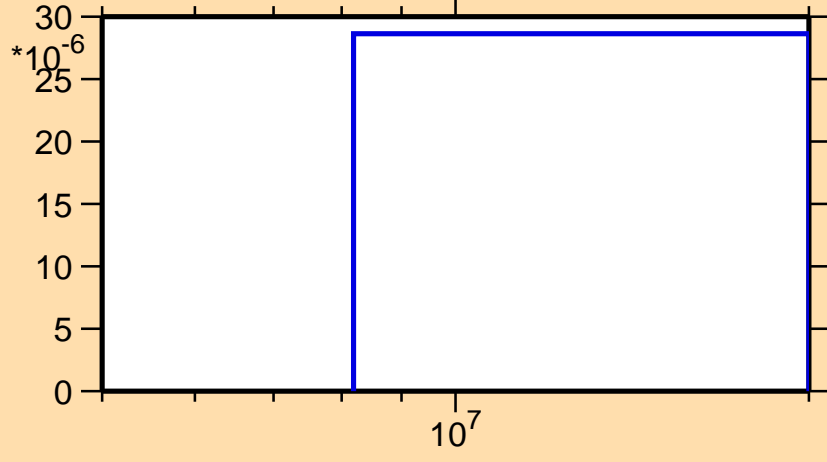
\sigma vs. E for ^{112}\text{Pd}(n,d)
