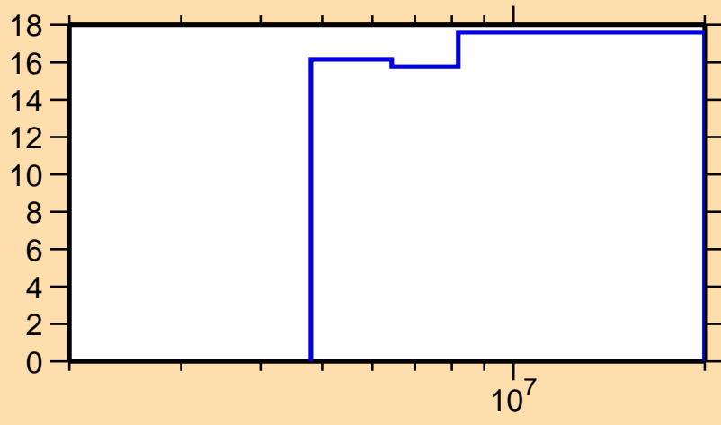
\Delta\sigma/\sigma vs. E for ^{112}\text{Pd}(n,n_1)
