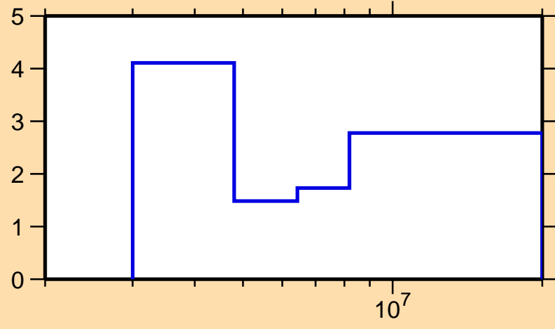
\Delta\sigma/\sigma vs. E for ^{112}\text{Pd}(n,\text{tot.})
