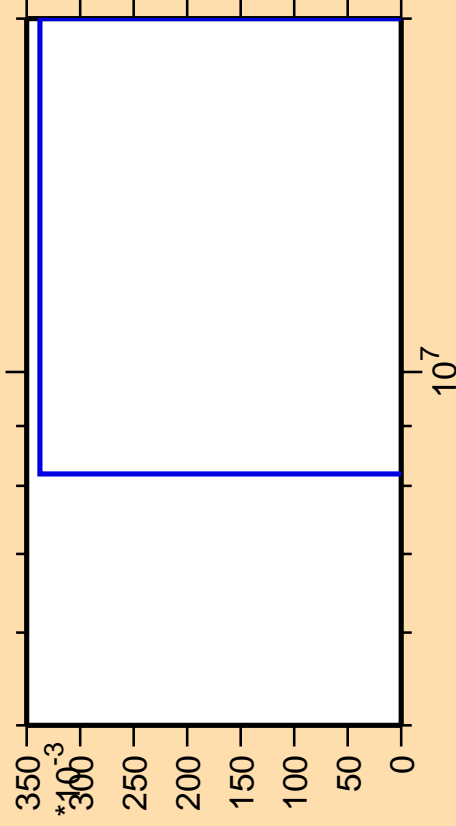
\Delta\sigma/\sigma vs. E for ^{112}\text{Pd}(n,\text{nd})
