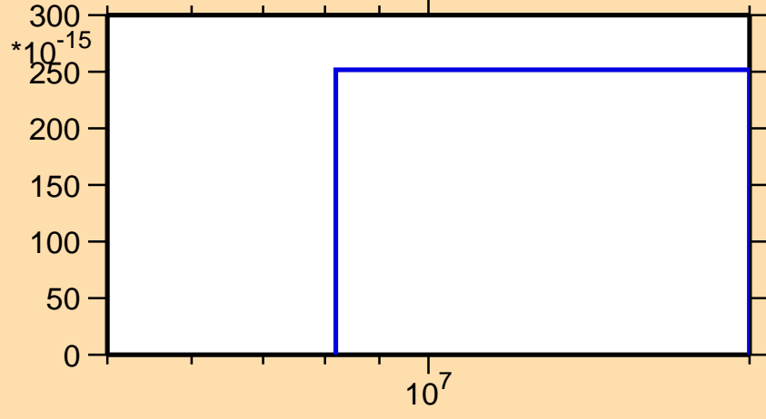
\sigma vs. E for ^{112}\text{Pd}(n,\text{nd})
