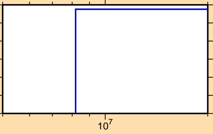
\sigma vs. E for ^{112}\text{Pd}(n,t)
