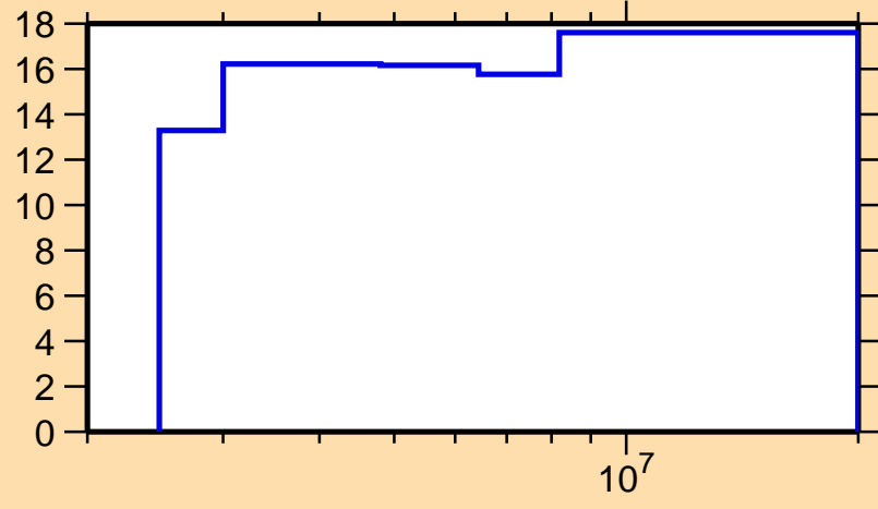
\Delta\sigma/\sigma vs. E for ^{112}\text{Pd}(n,n_1)
