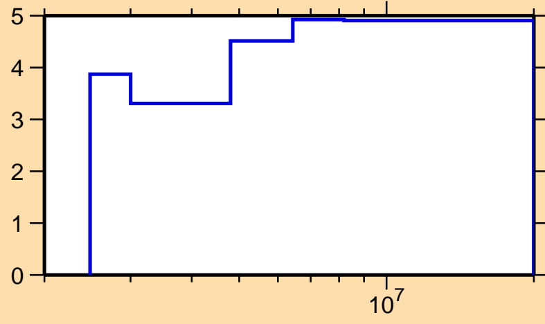
\Delta\sigma/\sigma vs. E for ^{112}\text{Pd}(n,\text{el.})
