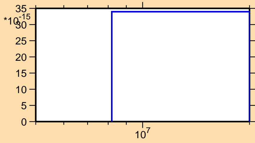
\sigma vs. E for ^{112}\text{Pd}(n,2n\alpha)
