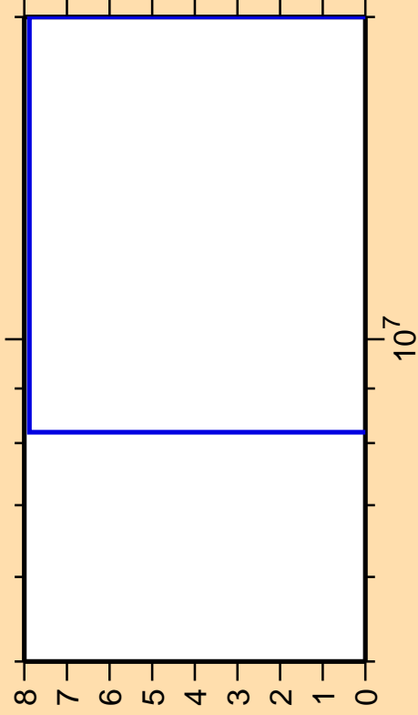
\Delta\sigma/\sigma vs. E for ^{112}\text{Pd}(n,2n)
