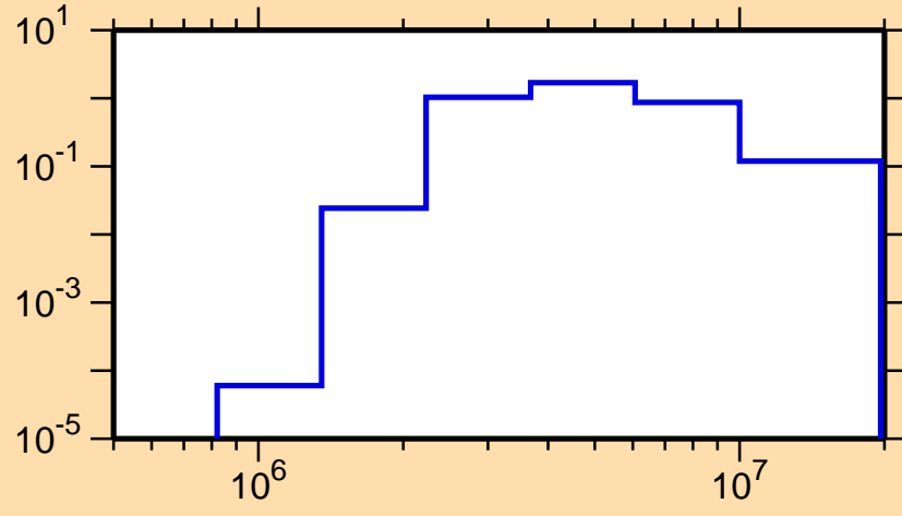
\sigma vs. E for ^{113}\text{Pd}(n,n\text{cont.})
