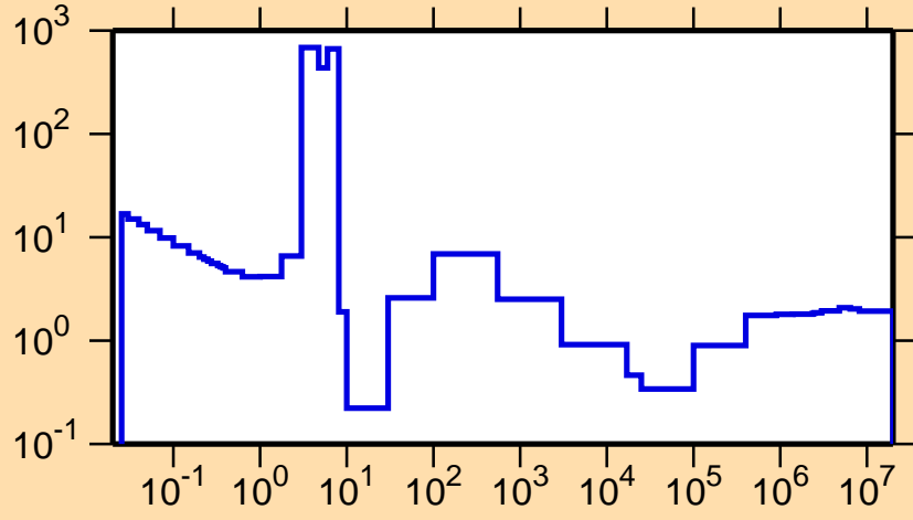
\sigma vs. E for ^{113}\text{Pd}(n,\text{nonel.})
