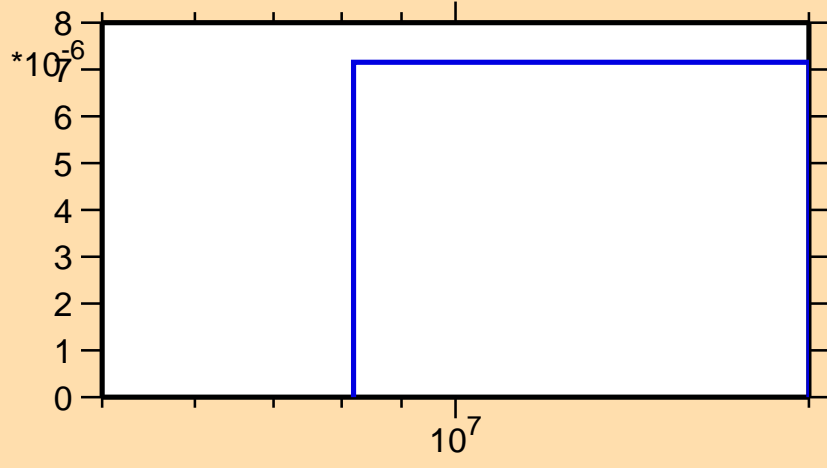
\sigma vs. E for ^{113}\text{Pd}(n,t)
