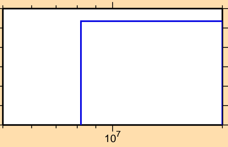
\sigma vs. E for ^{113}\text{Pd}(n,3n)
