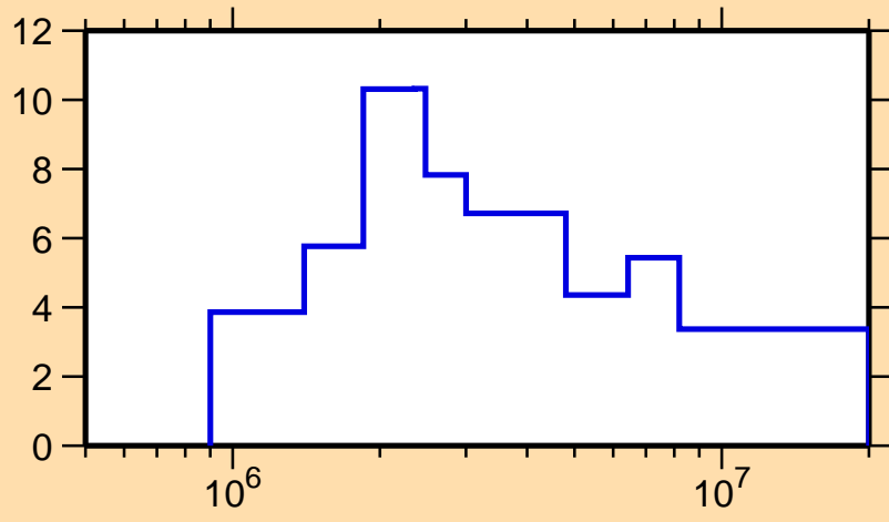
\Delta\sigma/\sigma vs. E for ^{113}\text{Pd}(n, el.)
