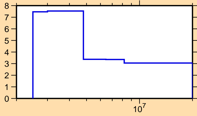
\Delta\sigma/\sigma vs. E for ^{113}\text{Pd}(n,\text{tot.})
