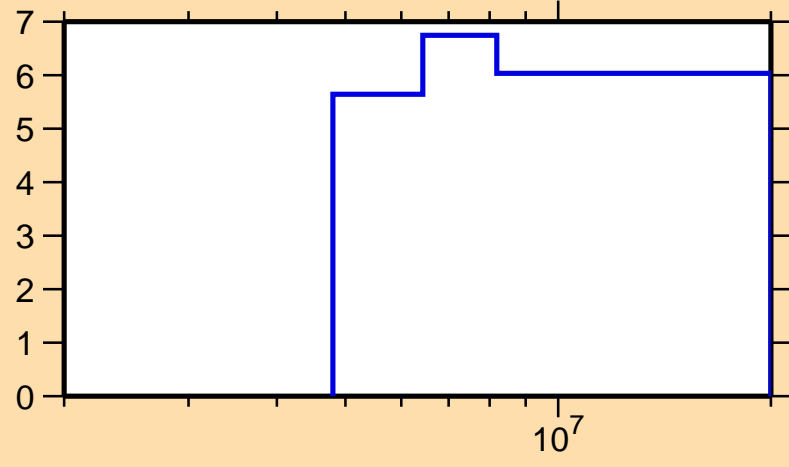
\Delta\sigma/\sigma vs. E for ^{113}\text{Pd}(n,\text{nonel.})
