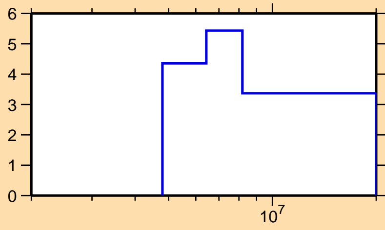
\Delta\sigma/\sigma vs. E for ^{113}\text{Pd}(n,\text{el.})
