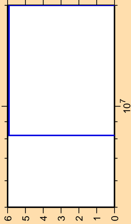
\Delta\sigma/\sigma vs. E for ^{113}\text{Pd}(n,2np)
