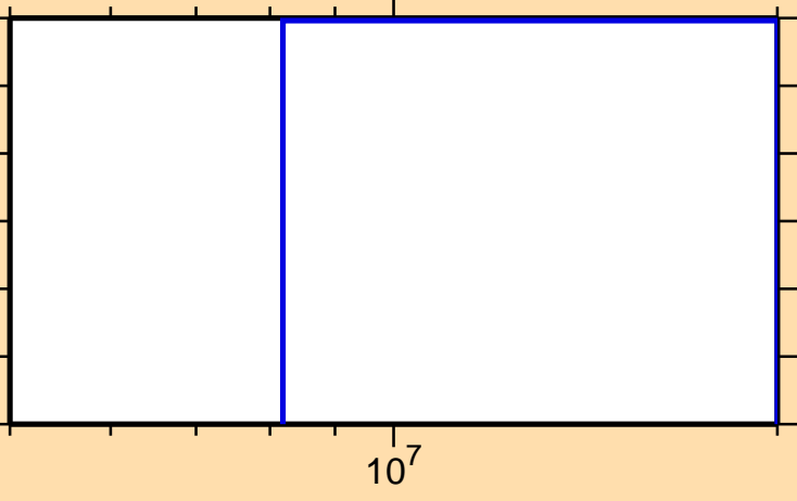
\sigma vs. E for ^{113}\text{Pd}(n,np)
