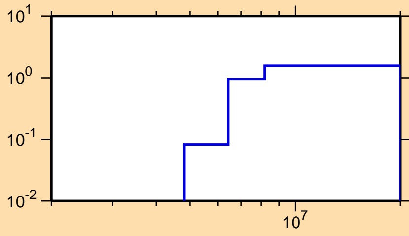
\sigma vs. E for ^{113}\text{Pd}(n,2n)
