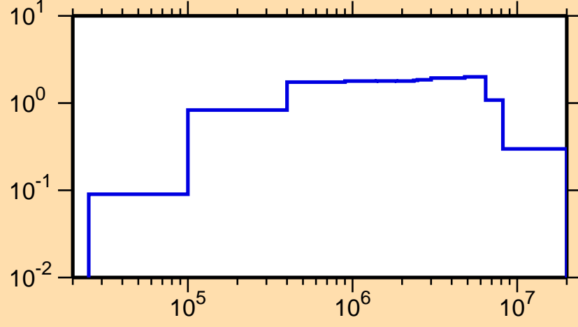
\sigma vs. E for ^{113}\text{Pd}(n,\text{inel.})
