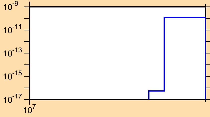
\sigma vs. E for ^{114}\text{Pd}(n,nt)
