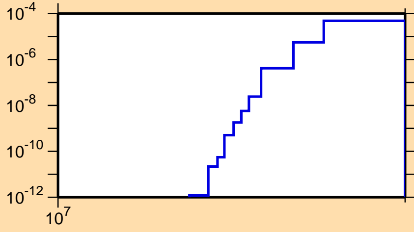
\sigma vs. E for ^{114}\text{Pd}(n,t)
