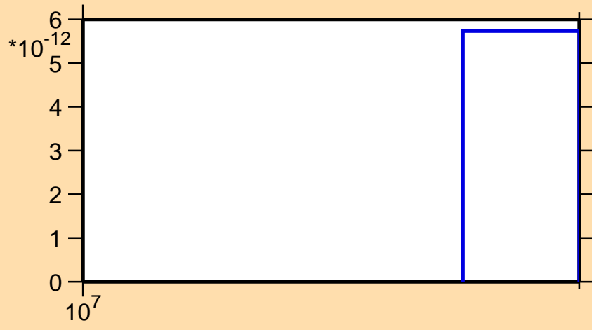
\sigma vs. E for ^{114}\text{Pd}(n,\text{nd})
