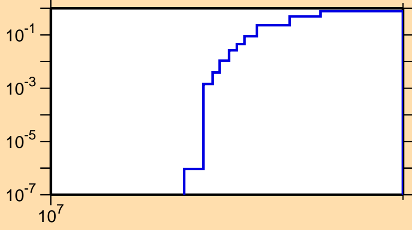
\sigma vs. E for ^{114}\text{Pd}(n,3n)
