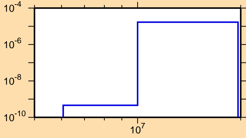
\sigma vs. E for ^{114}\text{Pd}(n,\alpha)
