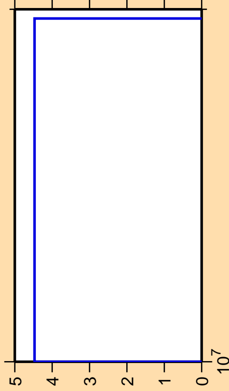
\Delta\sigma/\sigma vs. E for ^{114}\text{Pd}(n,nt)
