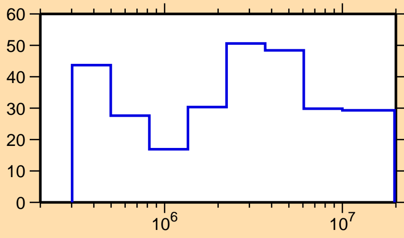
\Delta\sigma/\sigma vs. E for ^{114}\text{Pd}(n,n_1)
