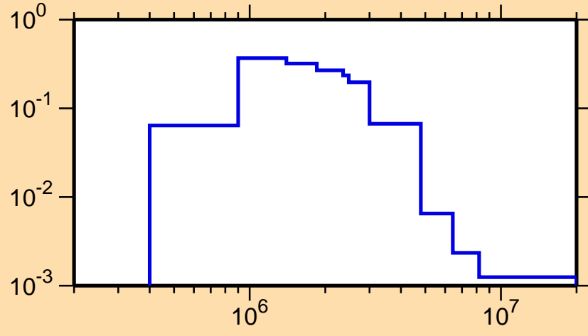
\sigma vs. E for ^{114}\text{Pd}(n,n_2)
