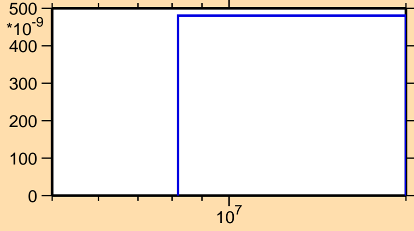
\sigma vs. E for ^{114}\text{Pd}(n,n\alpha)
