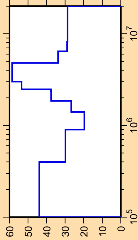
\Delta\sigma/\sigma vs. E for ^{114}\text{Pd}(n,n_1)
