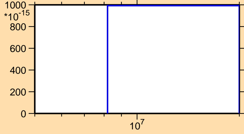
\sigma vs. E for ^{114}\text{Pd}(n,nt)
