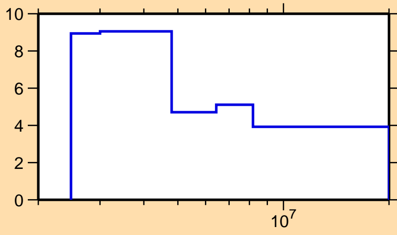
\Delta\sigma/\sigma vs. E for ^{114}\text{Pd}(n,n\text{onel.})
