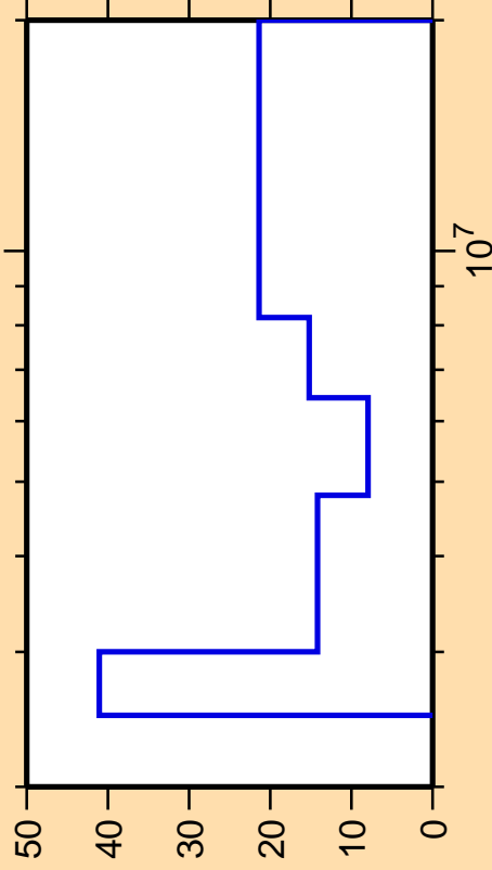
\Delta\sigma/\sigma vs. E for ^{114}\text{Pd}(n, n_{\text{cont}}) .
