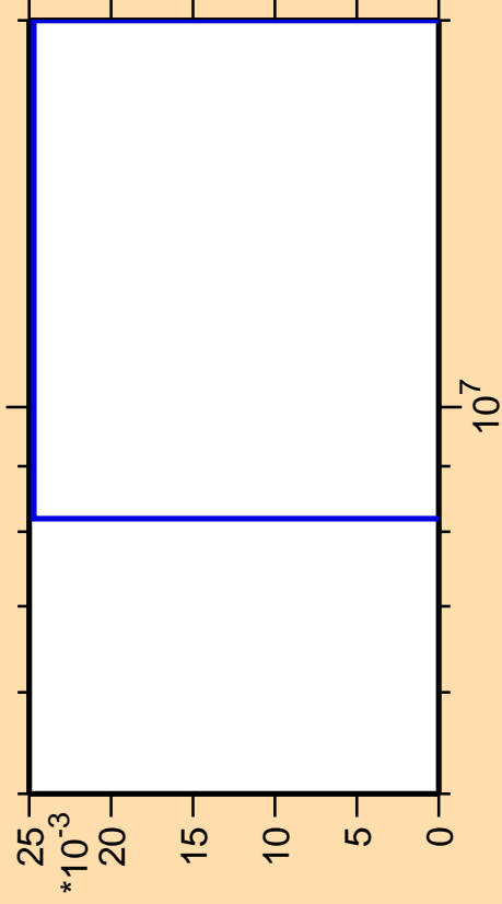
\Delta\sigma/\sigma vs. E for ^{114}\text{Pd}(n,2n\alpha)
