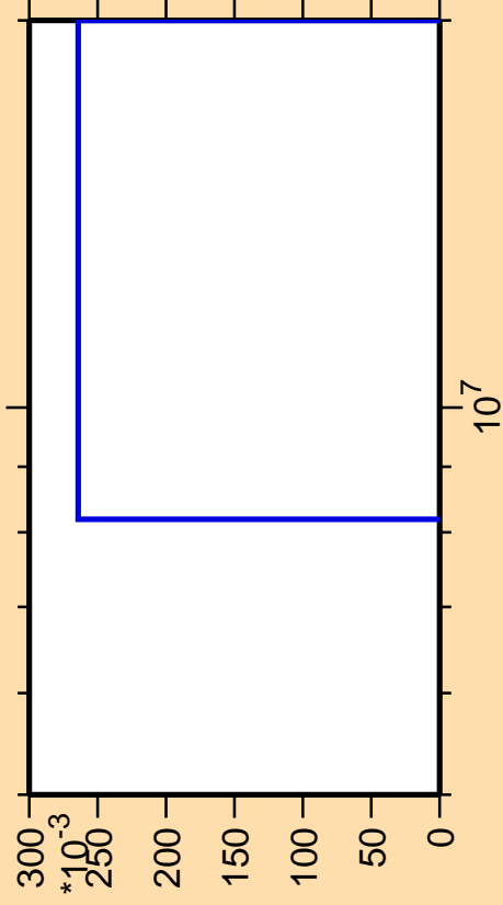
\Delta\sigma/\sigma vs. E for ^{114}\text{Pd}(n,\text{nd})
