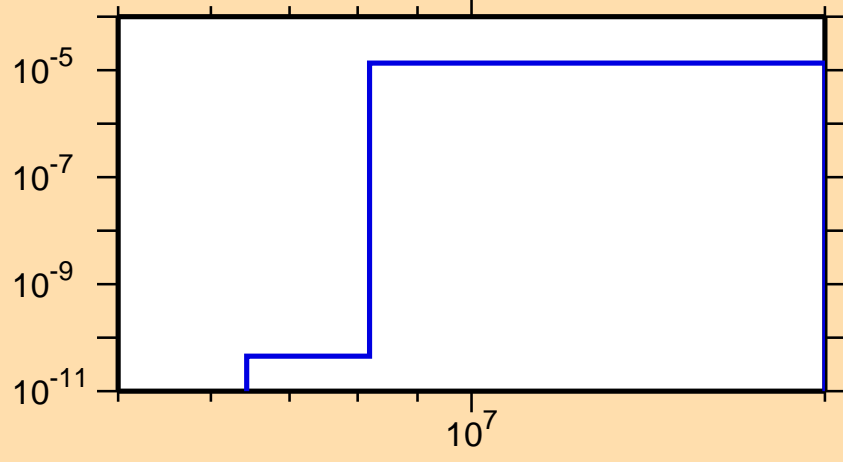
\sigma vs. E for ^{114}\text{Pd}(n,\alpha)
