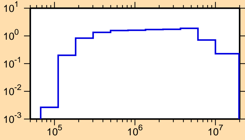
\sigma vs. E for ^{115}\text{Pd}(n,\text{inel.})
