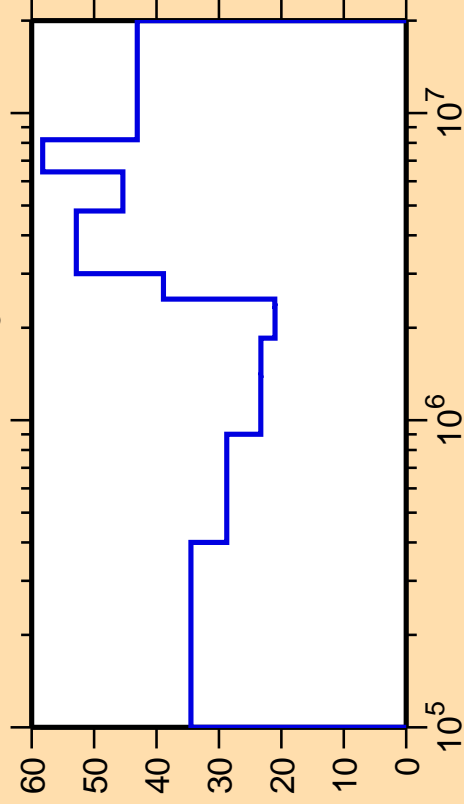
\Delta\sigma/\sigma vs. E for ^{115}\text{Pd}(n,n_3)
