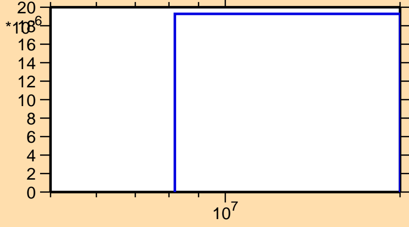
\sigma vs. E for ^{115}\text{Pd}(n,d)
