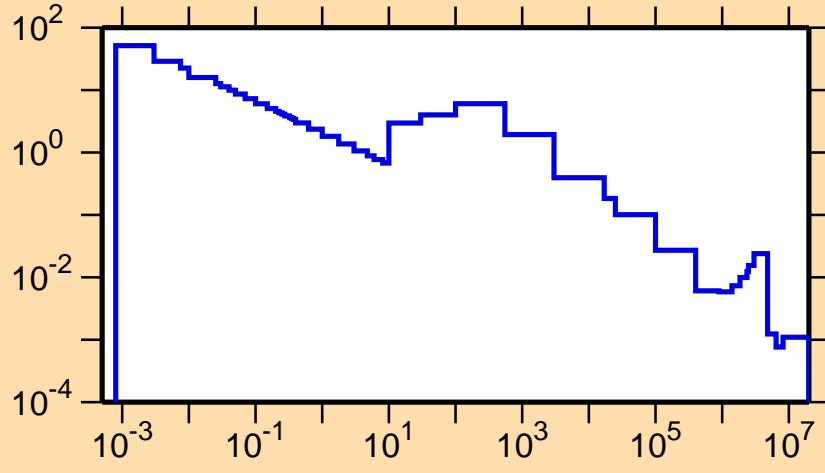
\sigma vs. E for ^{115}\text{Pd}(n,\gamma)
