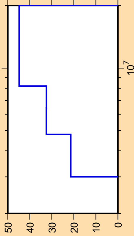
\Delta\sigma/\sigma vs. E for ^{115}\text{Pd}(n,\text{ncont.})
