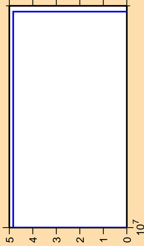
\Delta\sigma/\sigma vs. E for ^{115}\text{Pd}(n,2np)
