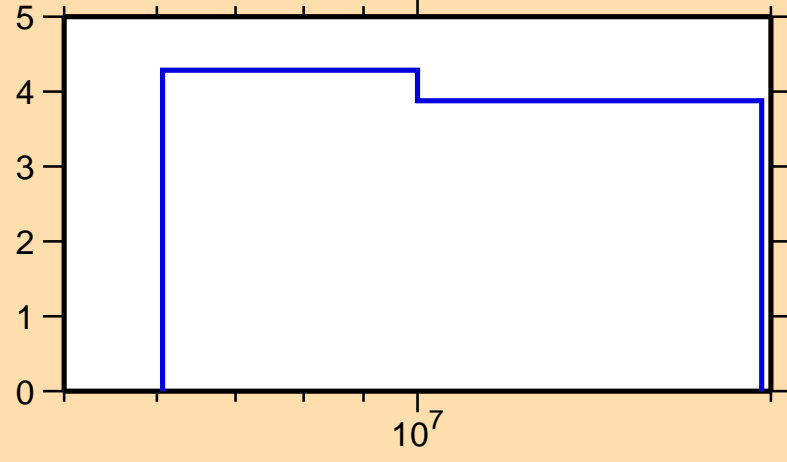
\Delta\sigma/\sigma vs. E for ^{116}\text{Pd}(n,\text{nonel.})
