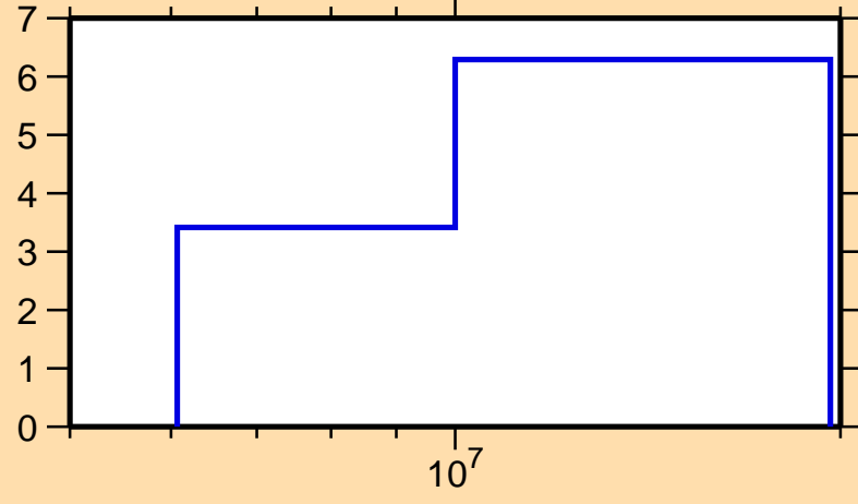
\Delta\sigma/\sigma vs. E for ^{116}\text{Pd}(n,\text{tot.})
