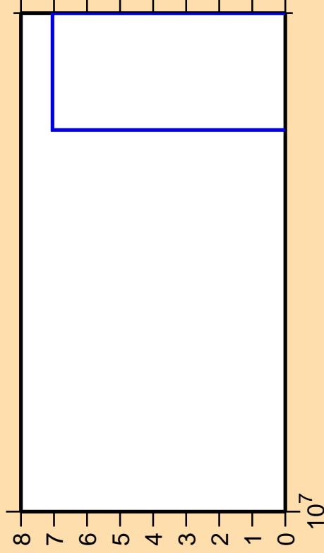
\Delta\sigma/\sigma vs. E for ^{117}\text{Pd}(n,2np)
