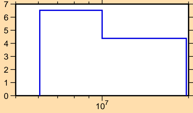
\Delta\sigma/\sigma vs. E for ^{117}\text{Pd}(n,\text{nonel.})
