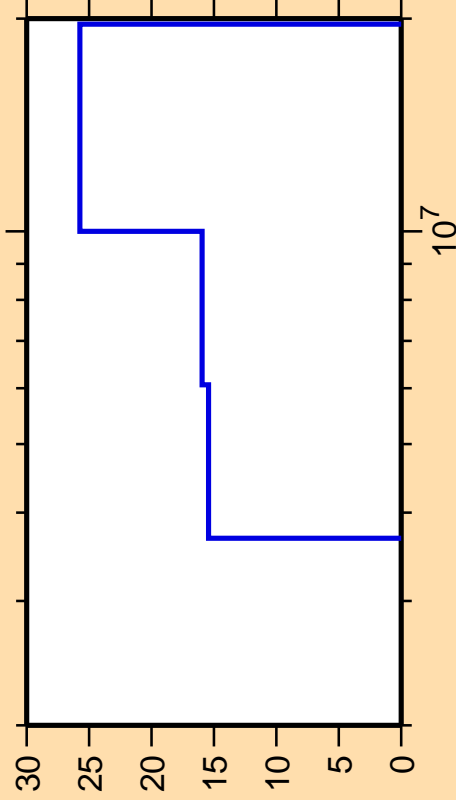
\Delta\sigma/\sigma vs. E for ^{117}\text{Pd}(n, n_{\text{cont}})
