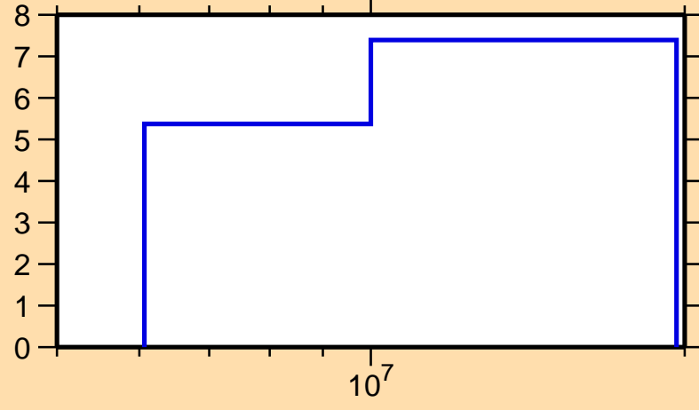
\Delta\sigma/\sigma vs. E for ^{117}\text{Pd}(n,\text{tot.})
