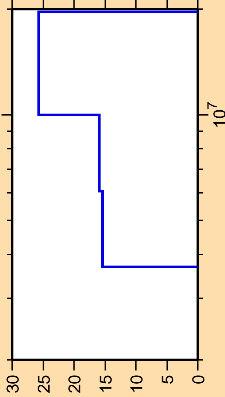
\Delta\sigma/\sigma vs. E for ^{117}\text{Pd}(n,n\text{cont.})
