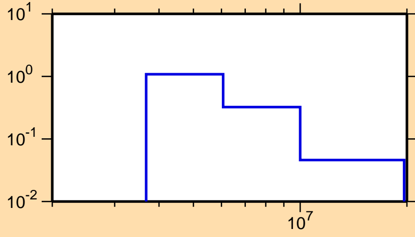
\sigma vs. E for ^{117}\text{Pd}(n,n\text{cont.})
