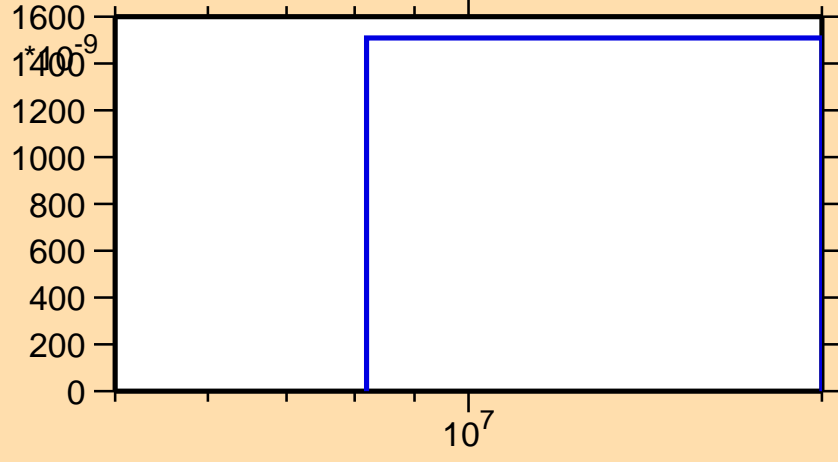
\sigma vs. E for ^{117}\text{Pd}(n,t)
