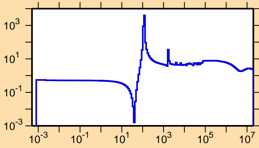
\sigma vs. E for ^{118}\text{Pd}(n,\text{el.})
