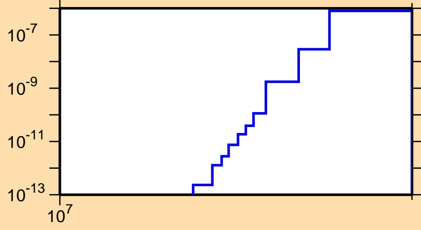
\sigma vs. E for ^{118}\text{Pd}(n,n\alpha)
