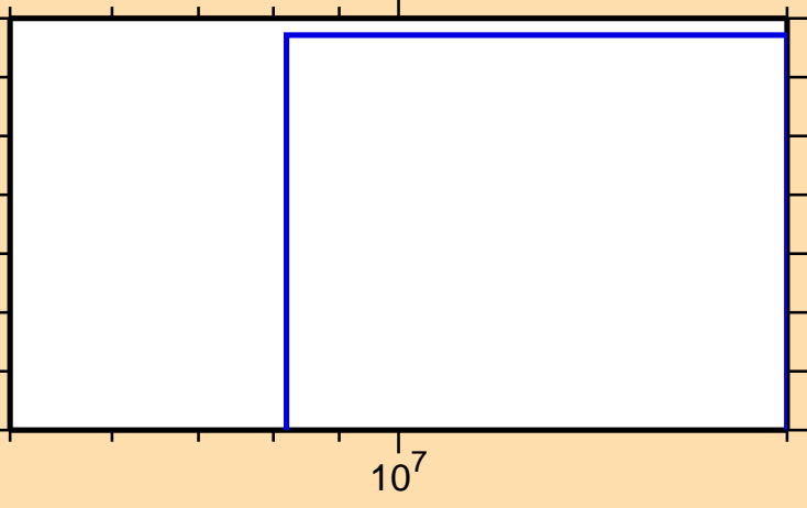
\sigma vs. E for ^{118}\text{Pd}(n,p)
