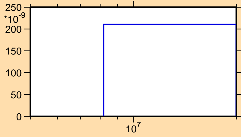
\sigma vs. E for ^{118}\text{Pd}(n,\alpha)
