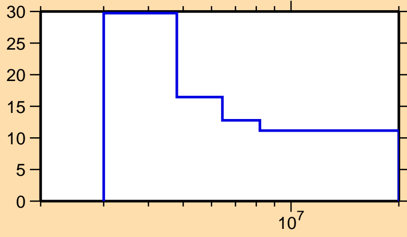
\Delta\sigma/\sigma vs. E for ^{118}\text{Pd}(n, el.)
