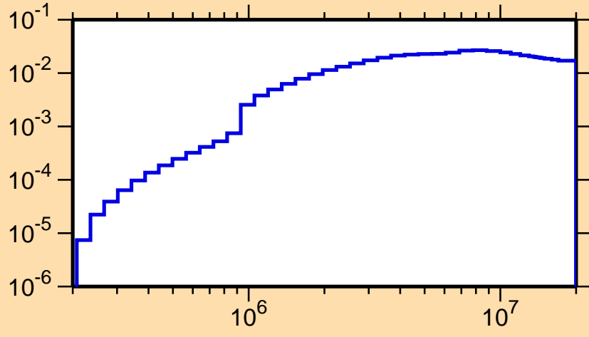
\sigma vs. E for ^{127}\text{Pm}(n,n\text{cont.})
