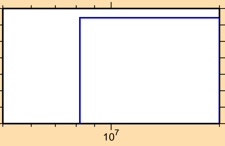
\sigma vs. E for ^{128}\text{Pm}(n,nt)
