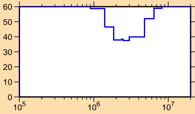
\Delta\sigma/\sigma vs. E for ^{128}\text{Pm}(n,n_1)
