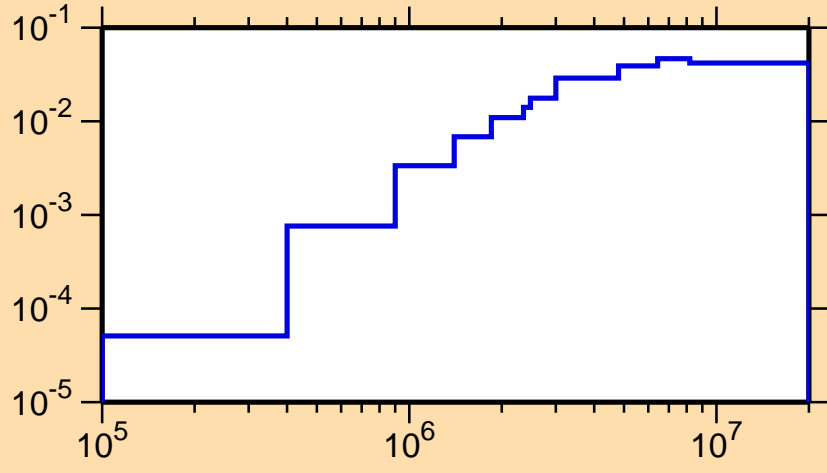
\sigma vs. E for ^{128}\text{Pm}(n,n\text{cont.})
