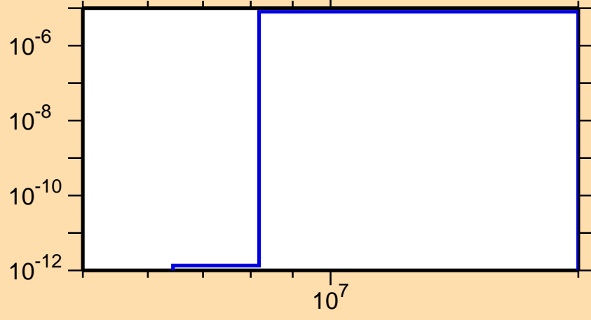
\sigma vs. E for ^{128}\text{Pm} (mt 45)
