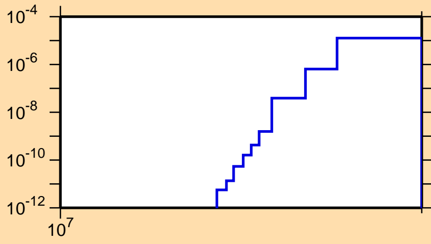
\sigma vs. E for ^{129}\text{Pm}(n,pt)
