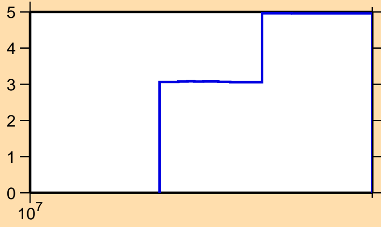
\Delta\sigma/\sigma vs. E for ^{129}\text{Pm}(n,\text{el.})
