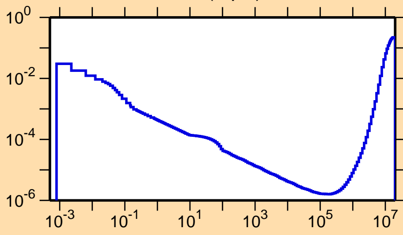
\sigma vs. E for ^{129}\text{Pm}(n,p\alpha)
