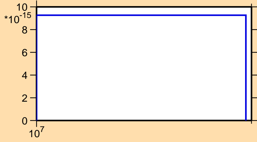
\sigma vs. E for ^{129}\text{Pm}(n,nt)
