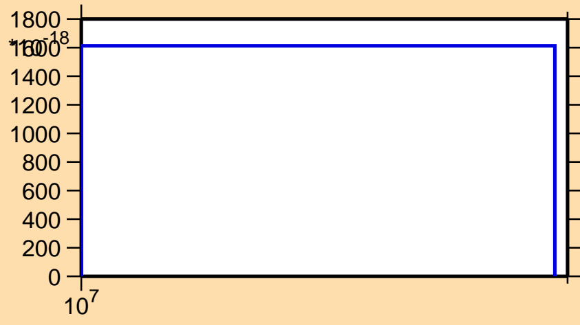
\sigma vs. E for ^{129}\text{Pm}(n,2n\alpha)
