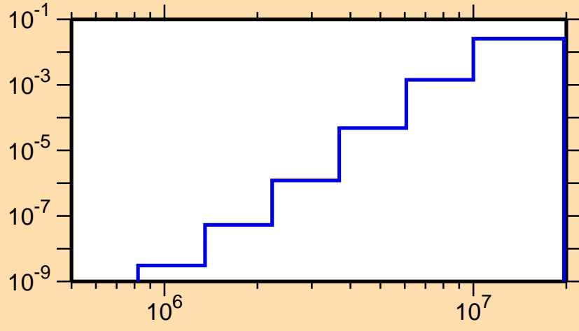
\sigma vs. E for ^{129}\text{Pm}(n,d)
