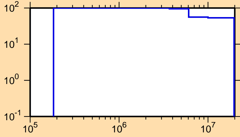
\Delta\sigma/\sigma vs. E for ^{129}\text{Pm}(n,ncont.)
