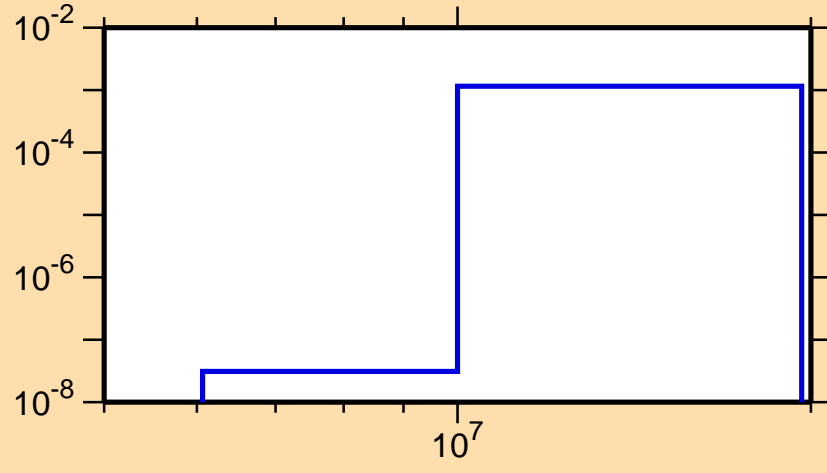
\sigma vs. E for ^{129}\text{Pm}(n,pd)
