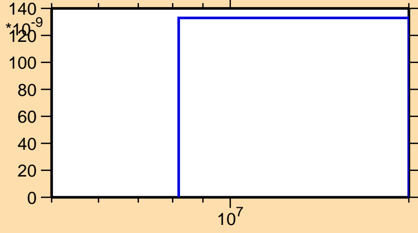
\sigma vs. E for ^{129}\text{Pm}(n,pt)
