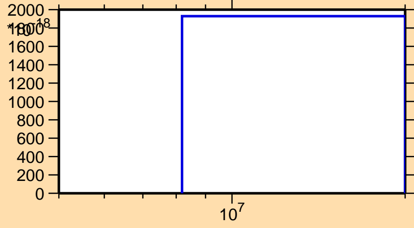
\sigma vs. E for ^{129}\text{Pm}(n,2n\alpha)
