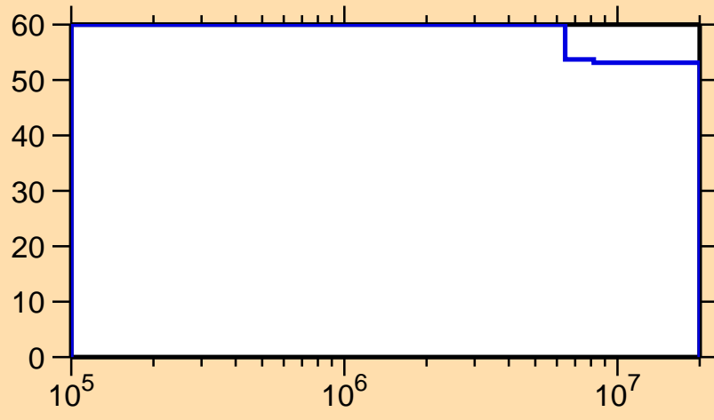
\Delta\sigma/\sigma vs. E for ^{129}\text{Pm}(n,n\text{cont.})
