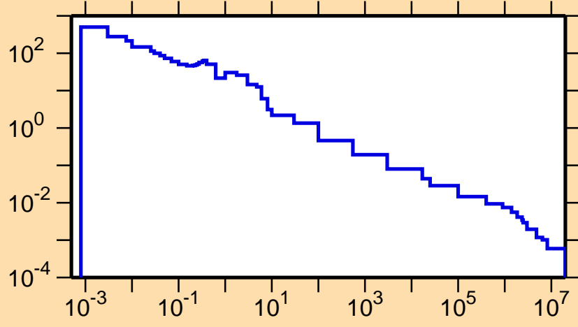
\sigma vs. E for ^{129}\text{Pm}(n,\gamma)
