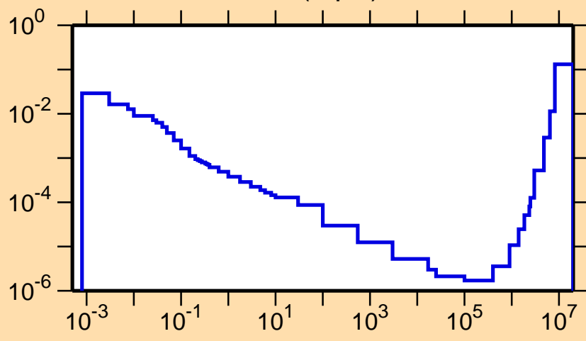
\sigma vs. E for ^{129}\text{Pm}(n,p\alpha)
