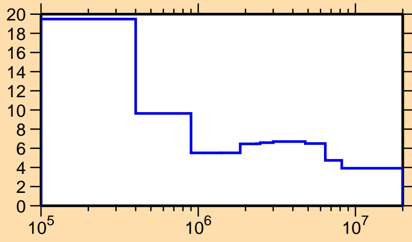
\Delta\sigma/\sigma vs. E for ^{129}\text{Pm}(n,\text{tot.})
