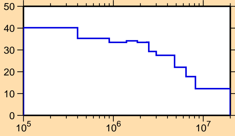
\Delta\sigma/\sigma vs. E for ^{129}\text{Pm}(n,n_1)
