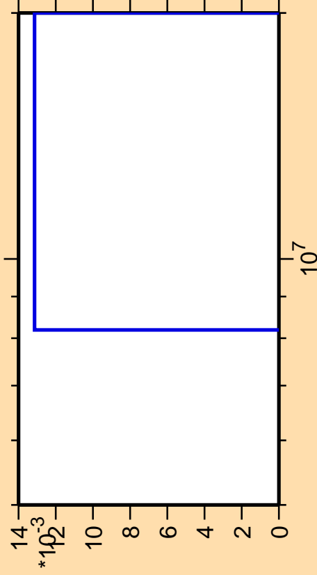
\Delta\sigma/\sigma vs. E for ^{129}\text{Pm}(n,2n\alpha)
