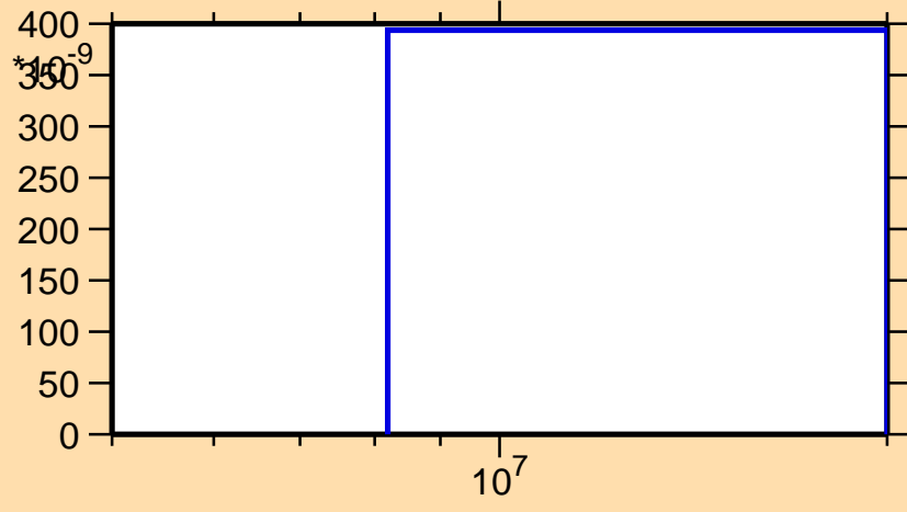
\sigma vs. E for ^{129}\text{Pm}(n,2np)
