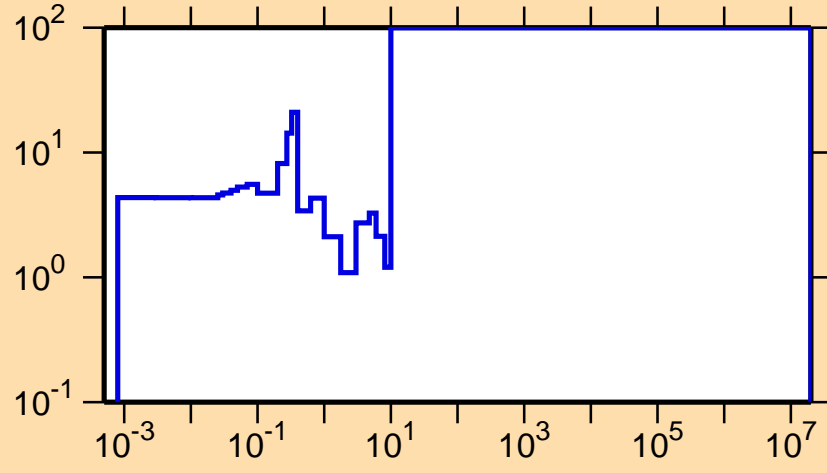
\Delta\sigma/\sigma vs. E for ^{129}\text{Pm}(n,\gamma)
