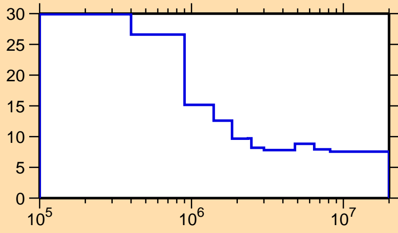
\Delta\sigma/\sigma vs. E for ^{129}\text{Pm}(n,\text{nonel.})
