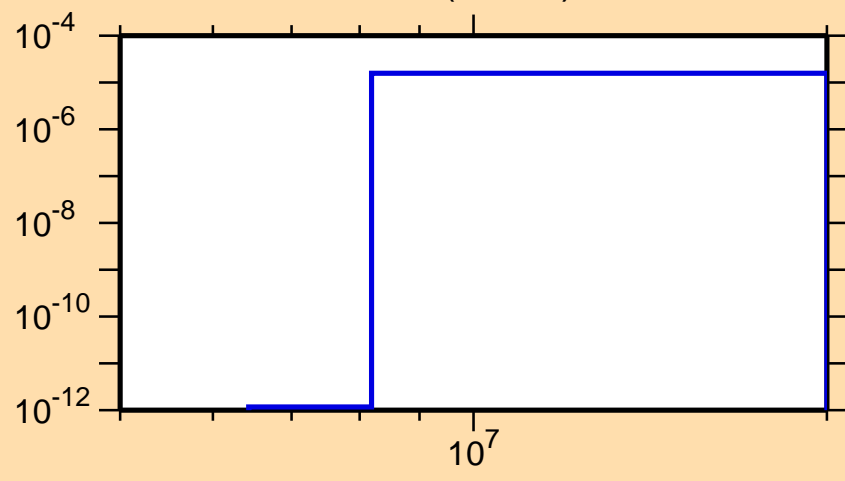
\sigma vs. E for ^{129}\text{Pm} (mt 45)
