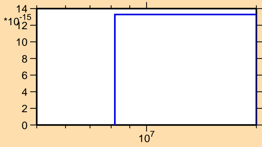
\sigma vs. E for ^{129}\text{Pm}(n,nt)
