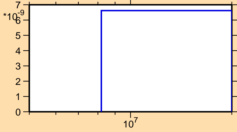
\sigma vs. E for ^{129}\text{Pm}(n,nd)
