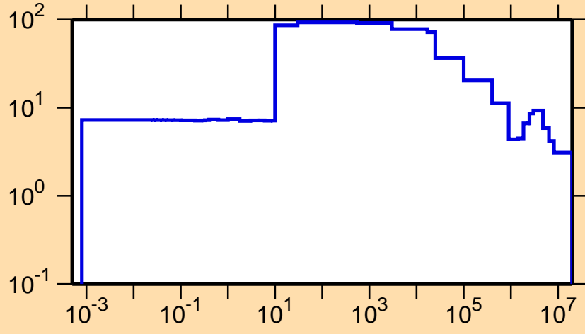
\Delta\sigma/\sigma vs. E for ^{129}\text{Pm}(n,el.)
