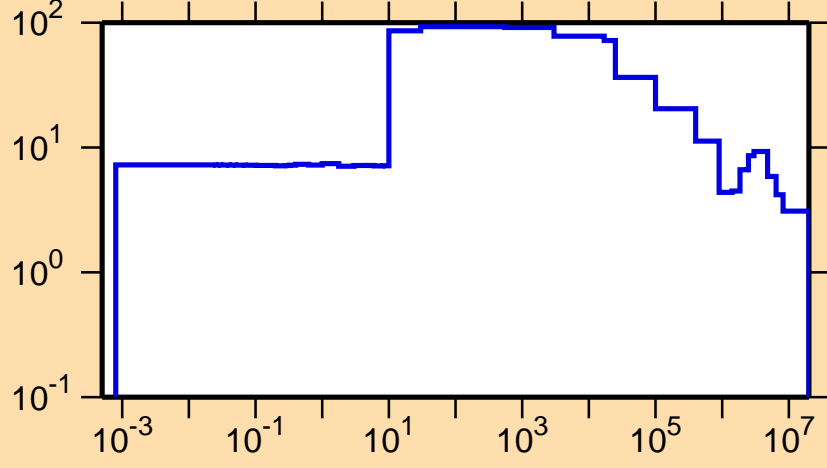
\Delta\sigma/\sigma vs. E for ^{129}\text{Pm}(n,\text{el.})
