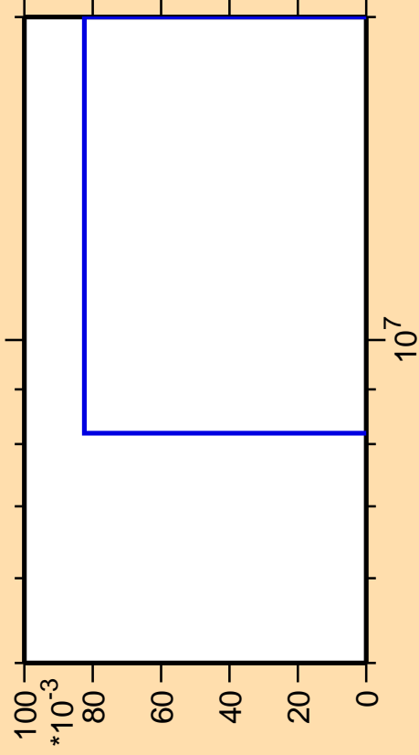
\Delta\sigma/\sigma vs. E for ^{129}\text{Pm}(n,nt)
