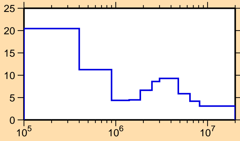
\Delta\sigma/\sigma vs. E for ^{129}\text{Pm}(n,el.)
