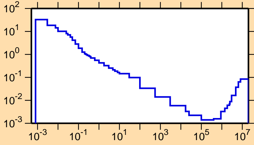
\sigma vs. E for ^{129}\text{Pm}(n,\alpha)
