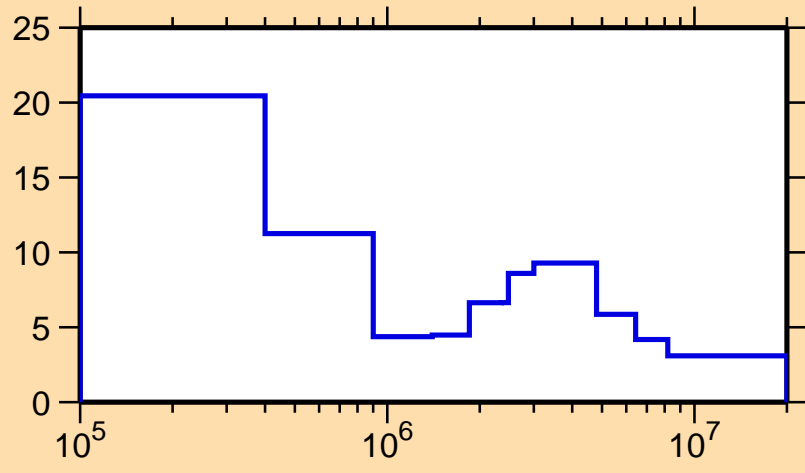
\Delta\sigma/\sigma vs. E for ^{129}\text{Pm}(n,\text{el.})
