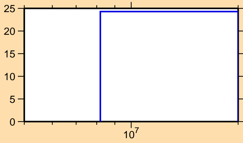
\Delta\sigma/\sigma vs. E for ^{129}\text{Pm}(n,\text{inel.})
