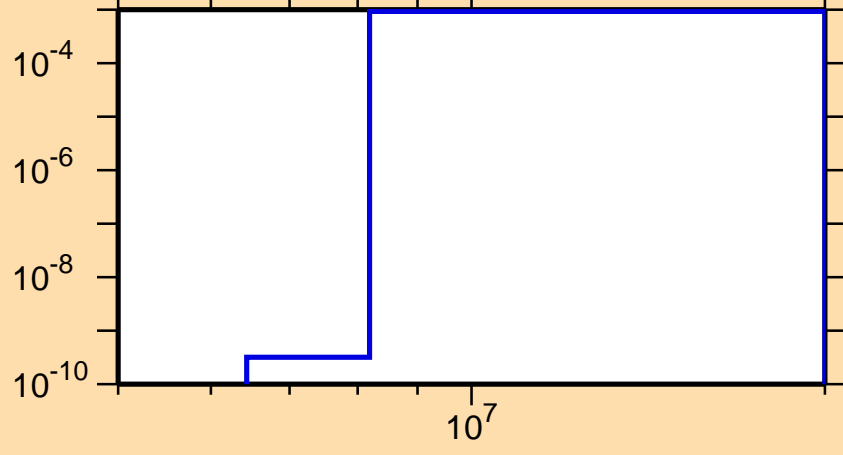
\sigma vs. E for ^{129}\text{Pm}(n,\text{pd})
