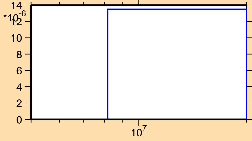
\sigma vs. E for ^{129}\text{Pm}(n,2n)
