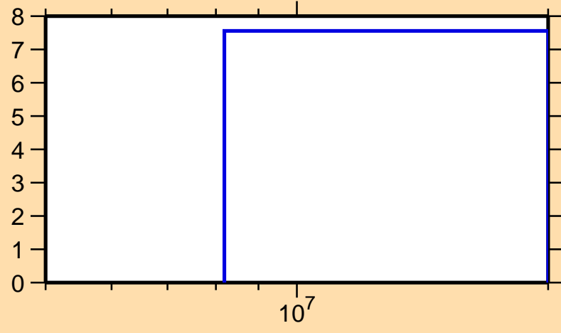
\Delta\sigma/\sigma vs. E for ^{129}\text{Pm}(n,\text{nonel.})
