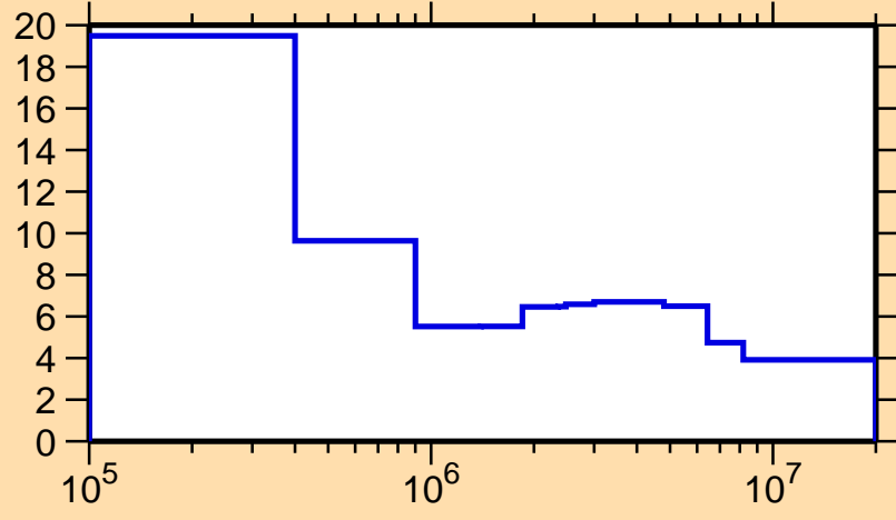
\Delta\sigma/\sigma vs. E for ^{129}\text{Pm}(n,\text{tot.})
