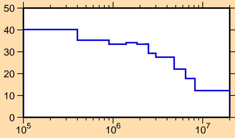
\Delta\sigma/\sigma vs. E for ^{129}\text{Pm}(n,n_1)
