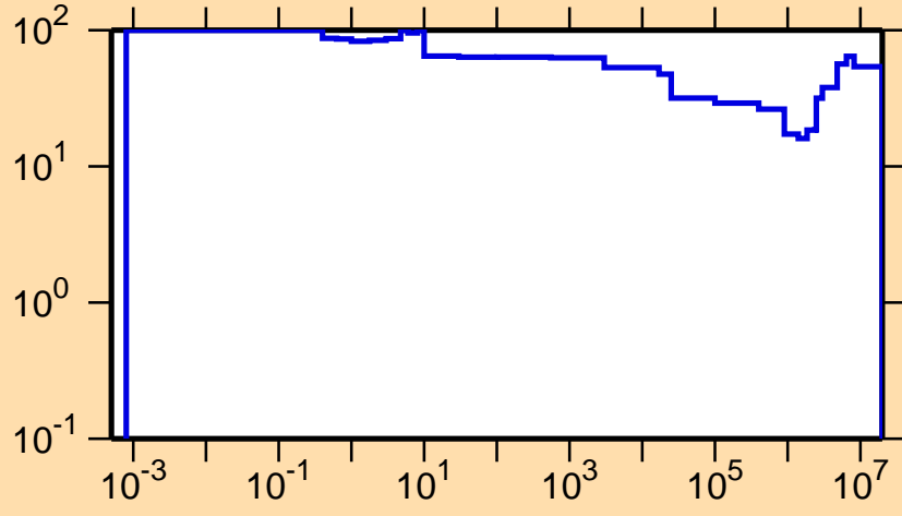
\Delta\sigma/\sigma vs. E for ^{129}\text{Pm}(n,p)
