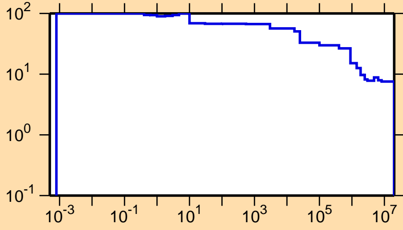
\Delta\sigma/\sigma vs. E for ^{129}\text{Pm}(n,\text{nonel.})
