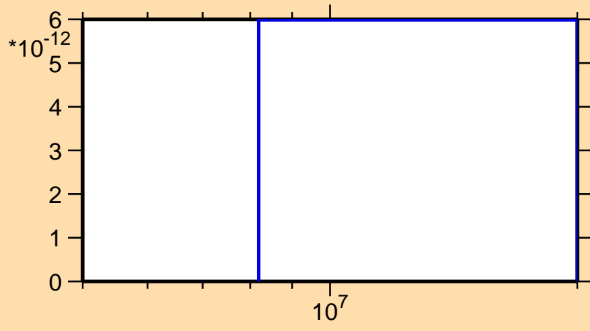
\sigma vs. E for ^{129}\text{Pm} (mt 34)
