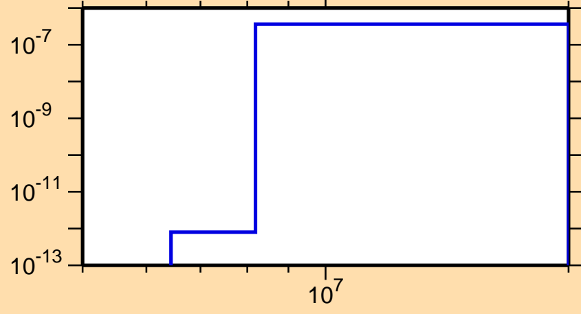
\sigma vs. E for ^{129}\text{Pm}(\text{mt117})
