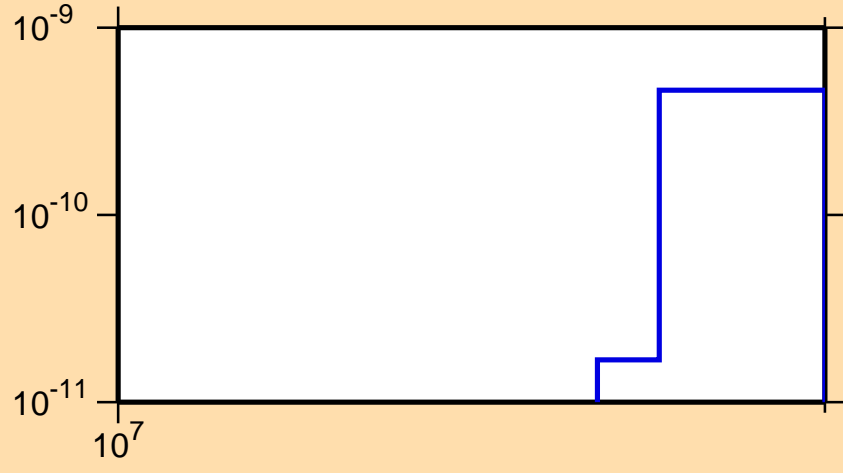
\sigma vs. E for ^{130}\text{Pm}(n,2n\alpha)
