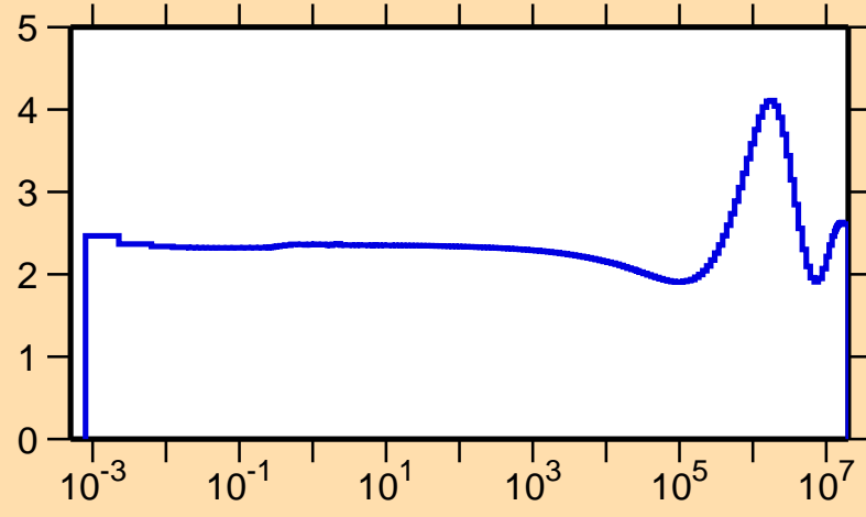
\sigma vs. E for ^{130}\text{Pm}(n,\text{el.})
