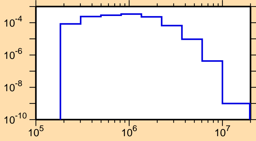
\sigma vs. E for ^{130}\text{Pm}(n,n_1)
