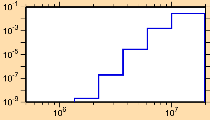
\sigma vs. E for ^{130}\text{Pm}(n,d)
