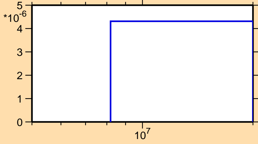
\sigma vs. E for ^{130}\text{Pm}(n,pt)
