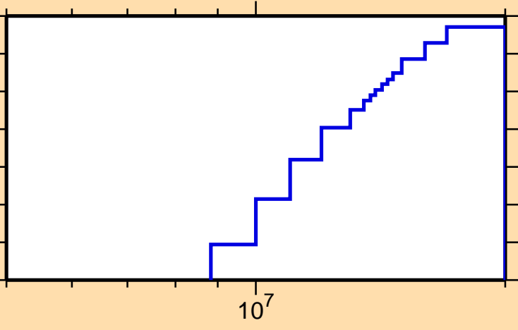
\sigma vs. E for ^{131}\text{Pm}(\text{mt117})
