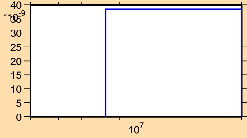
\sigma vs. E for ^{131}\text{Pm}(n,nd)
