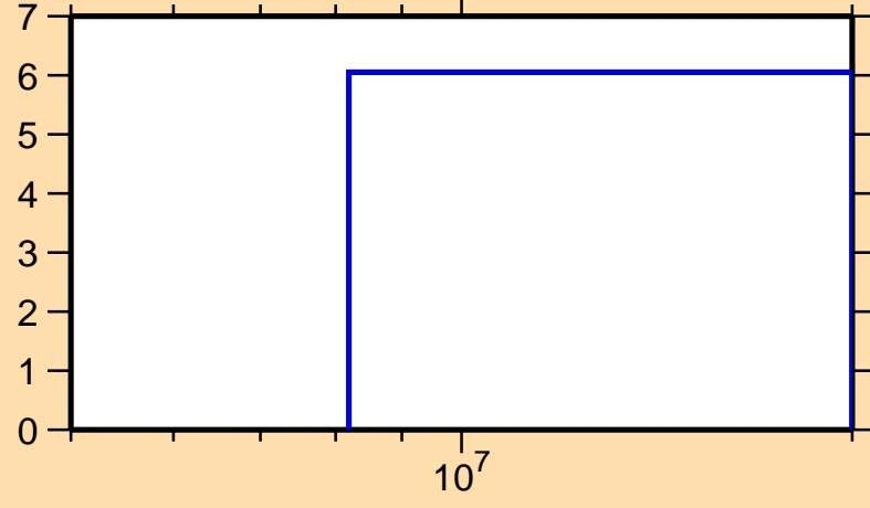
\Delta\sigma/\sigma vs. E for ^{132}\text{Pm}(n,\text{el.})
