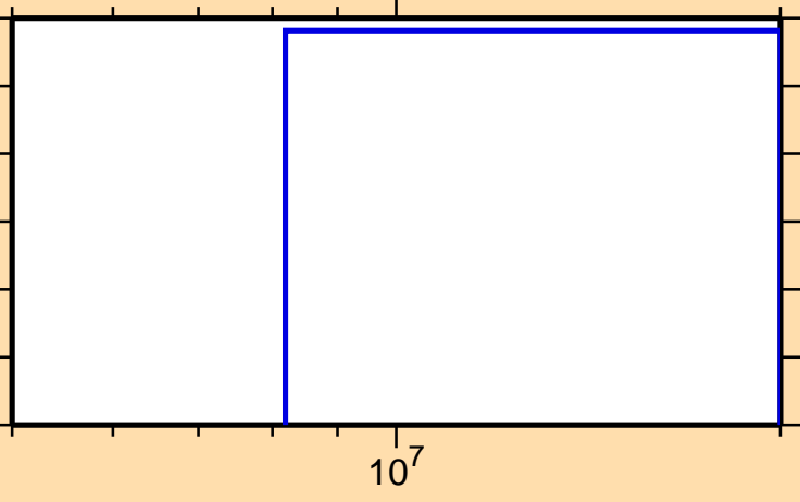
\sigma vs. E for ^{132}\text{Pm} (mt 45)
