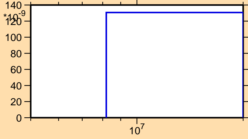
\sigma vs. E for ^{132}\text{Pm}(n,pt)
