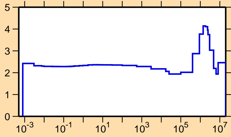
\sigma vs. E for ^{132}\text{Pm}(n,\text{el.})
