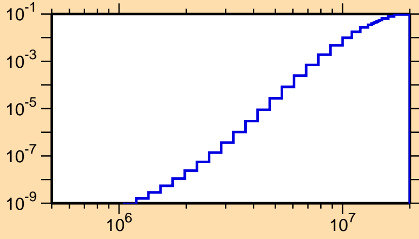
\sigma vs. E for ^{133}\text{Pm}(n,p\alpha)
