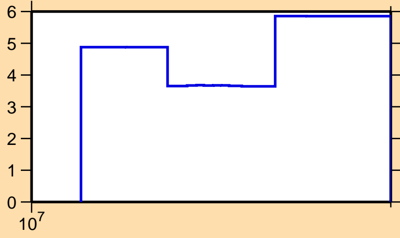
\Delta\sigma/\sigma vs. E for ^{133}\text{Pm}(n,\text{el.})
