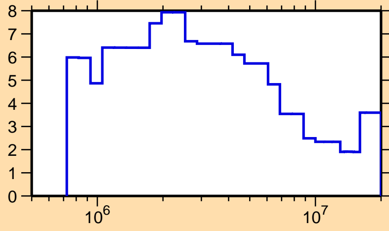
\Delta\sigma/\sigma vs. E for ^{133}\text{Pm}(n,\text{tot.})
