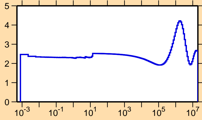
\sigma vs. E for ^{133}\text{Pm}(n,\text{el.})
