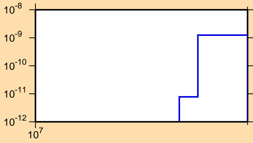
\sigma vs. E for ^{133}\text{Pm}(n,2n\alpha)
