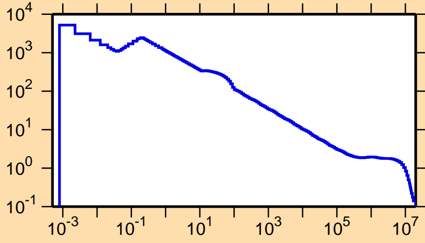
\sigma vs. E for ^{133}\text{Pm}(n,p)
