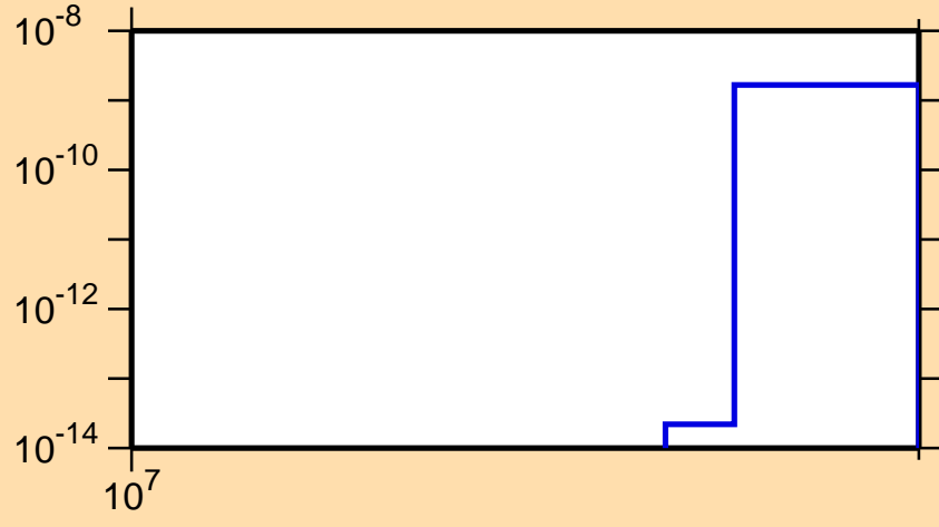
\sigma vs. E for ^{133}\text{Pm}(n,nt)
