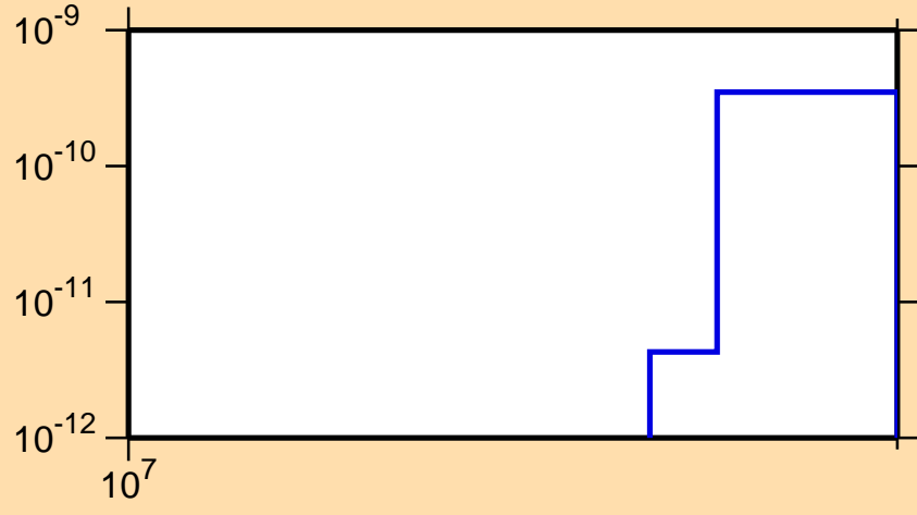
\sigma vs. E for ^{133}\text{Pm} (mt 34)
