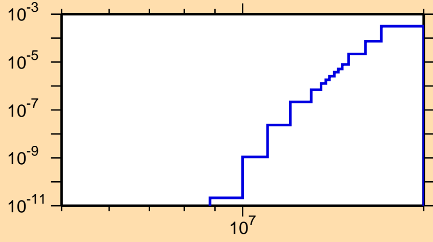
\sigma vs. E for ^{133}\text{Pm} (mt 45)
