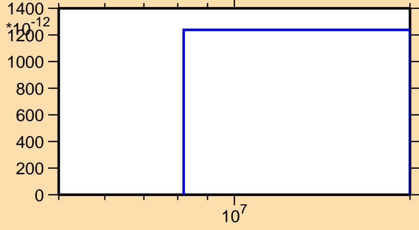
\sigma vs. E for ^{133}\text{Pm}(n,pt)
