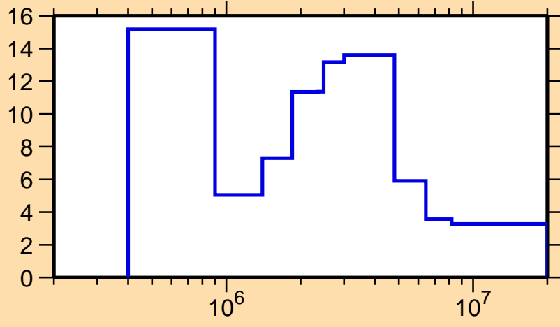
\Delta\sigma/\sigma vs. E for ^{133}\text{Pm}(n,\text{el.})
