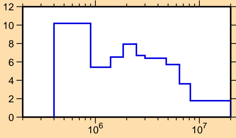
\Delta\sigma/\sigma vs. E for ^{133}\text{Pm}(n,\text{tot.})
