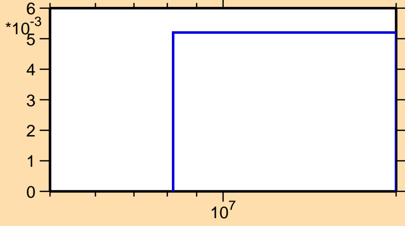
\sigma vs. E for ^{133}\text{Pm}(n,2n)
