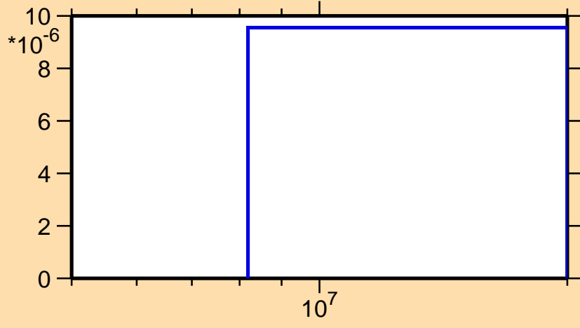
\sigma vs. E for ^{133}\text{Pm} (mt 45)
