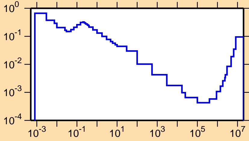
\sigma vs. E for ^{133}\text{Pm}(n,\alpha)
