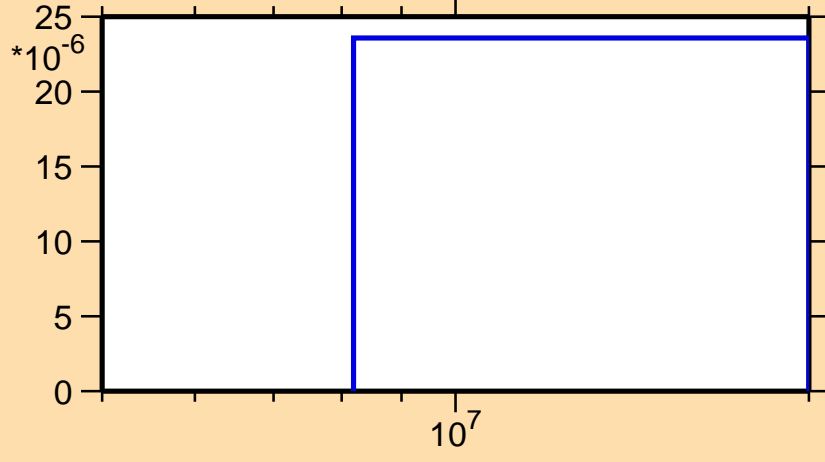
\sigma vs. E for ^{133}\text{Pm}(n,pd)
