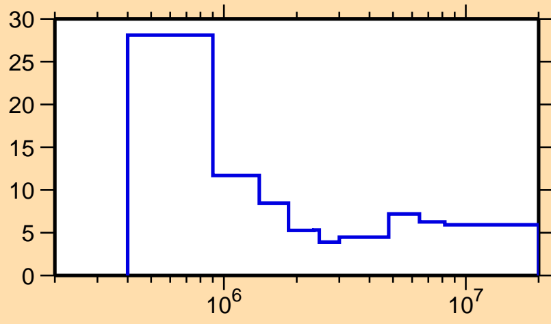
\Delta\sigma/\sigma vs. E for ^{133}\text{Pm}(n,\text{nonel.})
