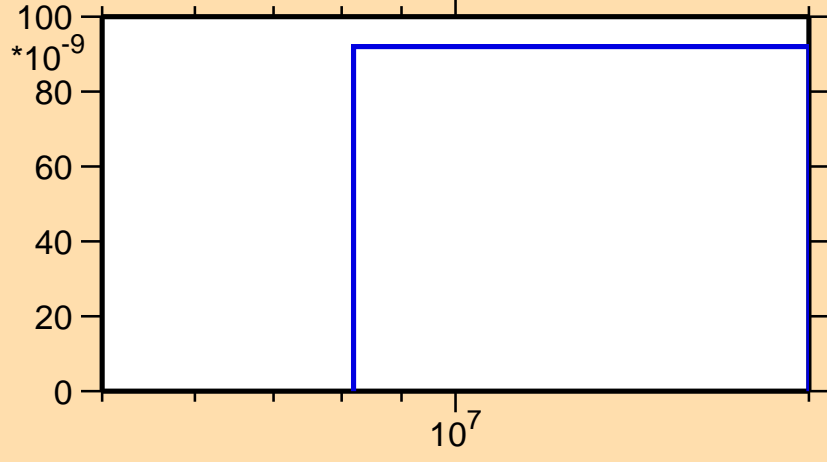
\sigma vs. E for ^{133}\text{Pm}(\text{mt117})
