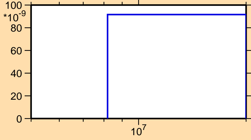
\sigma vs. E for ^{133}\text{Pm}(n,nd)
