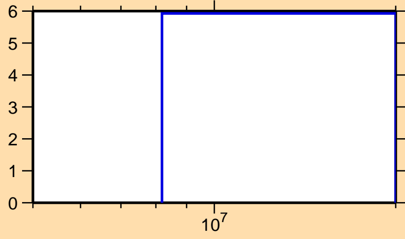
\Delta\sigma/\sigma vs. E for ^{133}\text{Pm}(n,\text{nonel.})
