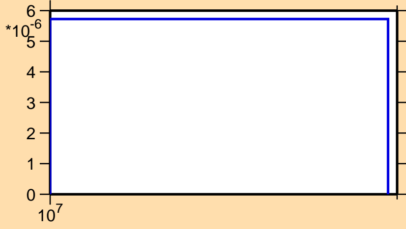
\sigma vs. E for ^{133}\text{Pm}(n,2np)
