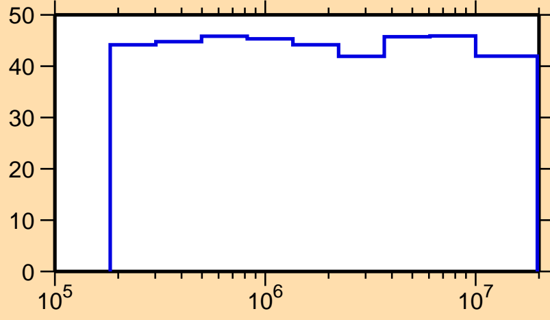
\Delta\sigma/\sigma vs. E for ^{133}\text{Pm}(n,n_1)
