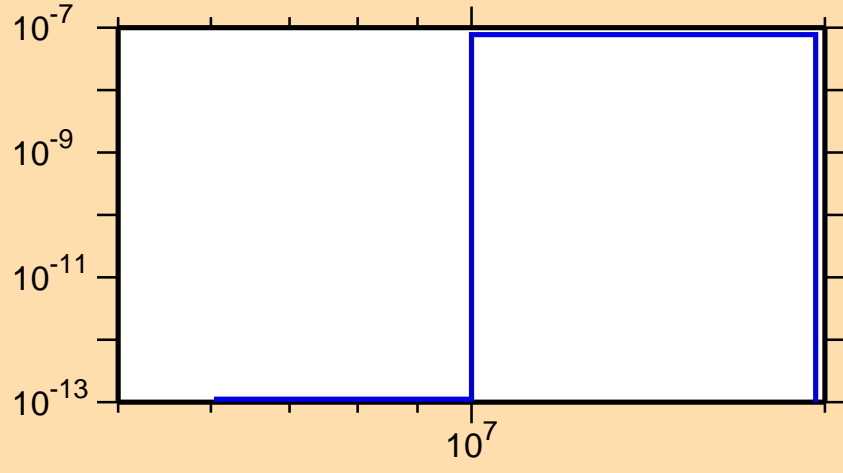
\sigma vs. E for ^{133}\text{Pm}(\text{mt117})
