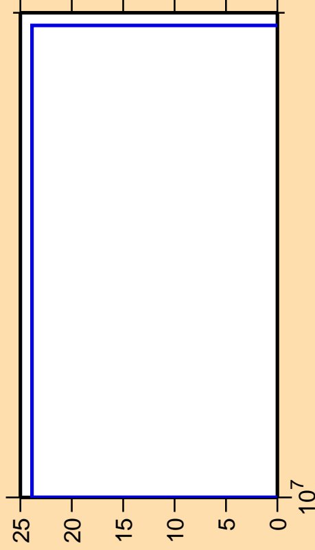
\Delta\sigma/\sigma vs. E for ^{133}\text{Pm} (mt 34)
