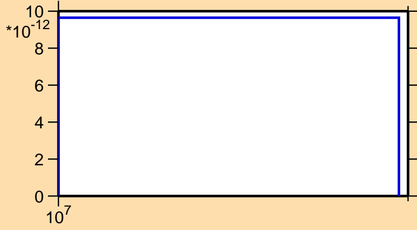
\sigma vs. E for ^{133}\text{Pm}(n,nt)
