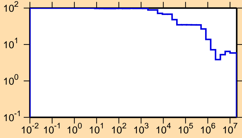
\Delta\sigma/\sigma vs. E for ^{133}\text{Pm}(n,\text{nonel.})
