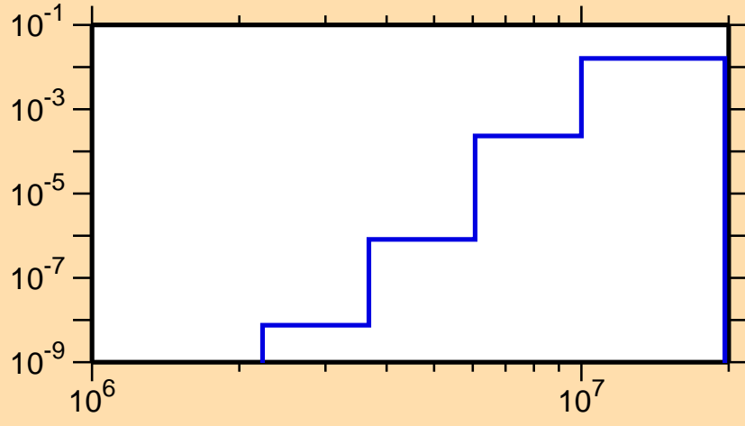
\sigma vs. E for ^{133}\text{Pm}(n,d)
