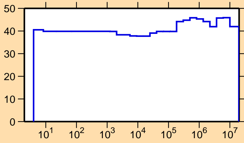
\Delta\sigma/\sigma vs. E for ^{133}\text{Pm}(n,n_1)
