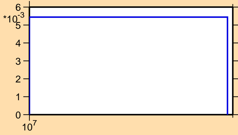
\sigma vs. E for ^{133}\text{Pm}(n,2n)
