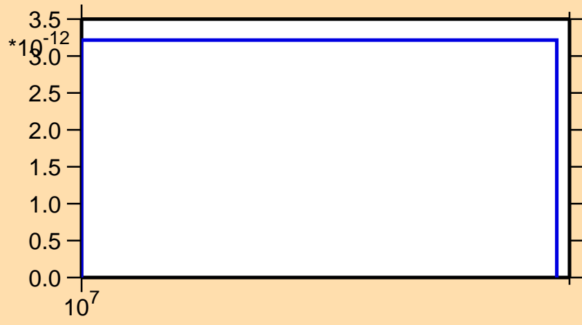
\sigma vs. E for ^{133}\text{Pm} (mt 34)
