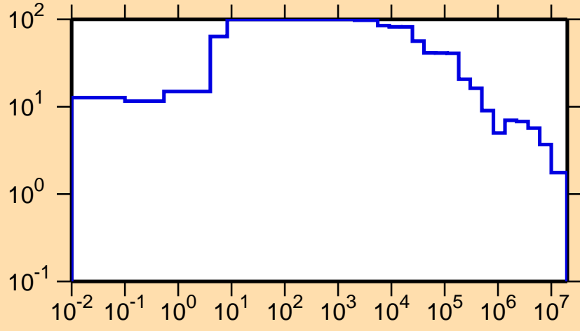
\Delta\sigma/\sigma vs. E for ^{133}\text{Pm}(n,\text{tot.})
