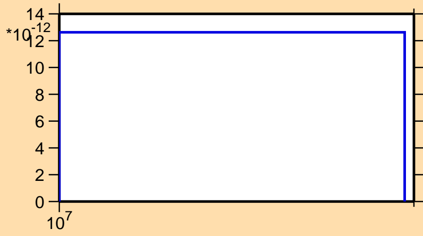
\sigma vs. E for ^{133}\text{Pm}(n,2n\alpha)
