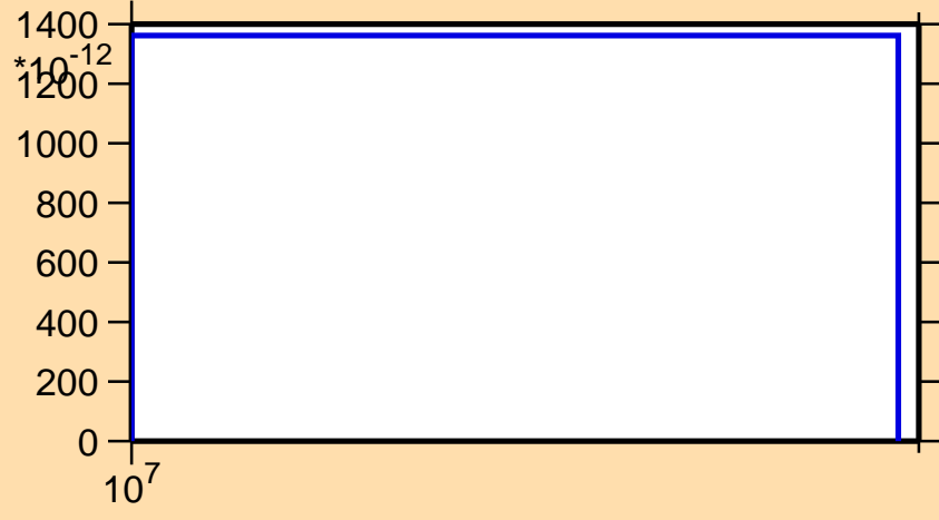
\sigma vs. E for ^{133}\text{Pm}(n,\text{pt})
