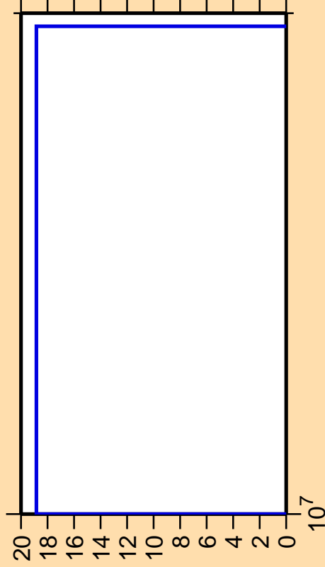
\Delta\sigma/\sigma vs. E for ^{133}\text{Pm}(n,n\text{cont.})
