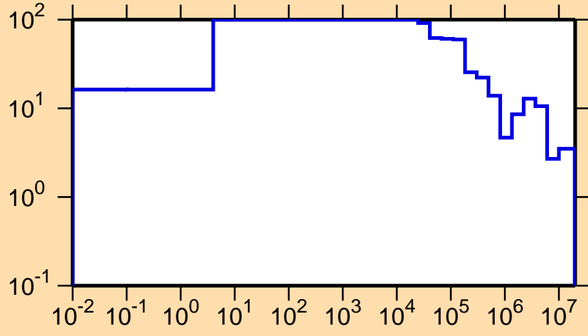
\Delta\sigma/\sigma vs. E for ^{133}\text{Pm}(n,el.)
