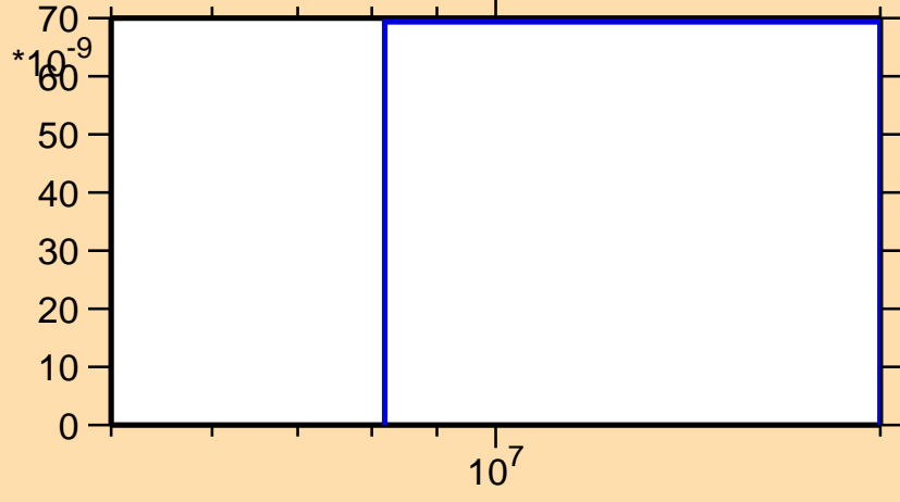
\sigma vs. E for ^{133}\text{Pm}(n,nd)
