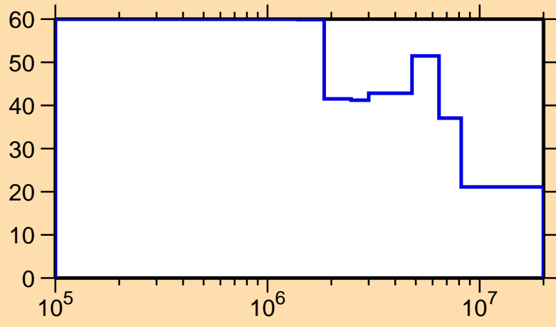
\Delta\sigma/\sigma vs. E for ^{133}\text{Pm}(n,n\text{cont.})
