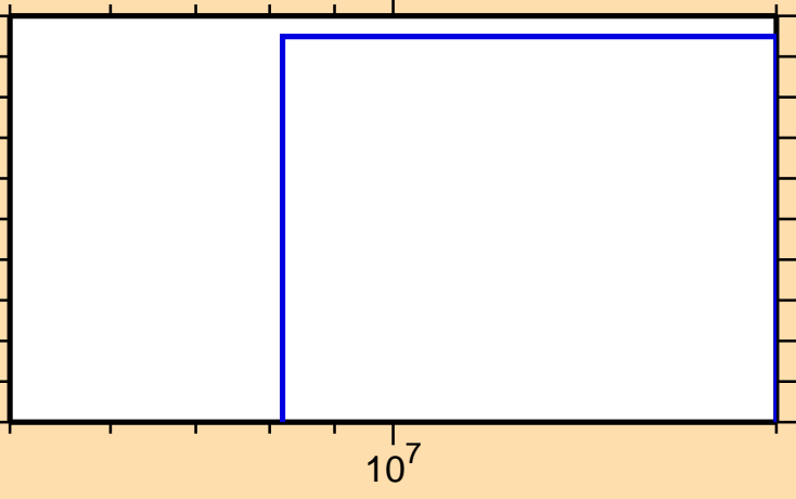
\sigma vs. E for ^{133}\text{Pm}(n,pd)
