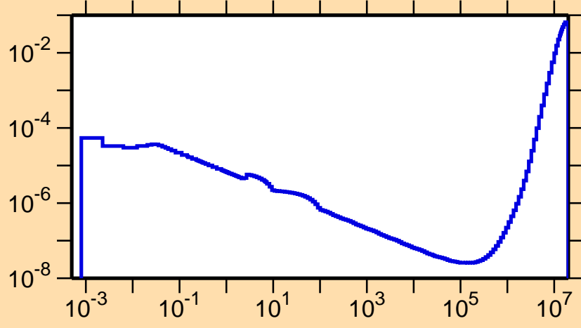
\sigma vs. E for ^{134}\text{Pm}(n,p\alpha)
