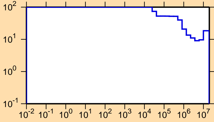
\Delta\sigma/\sigma vs. E for ^{134}\text{Pm}(n,p)
