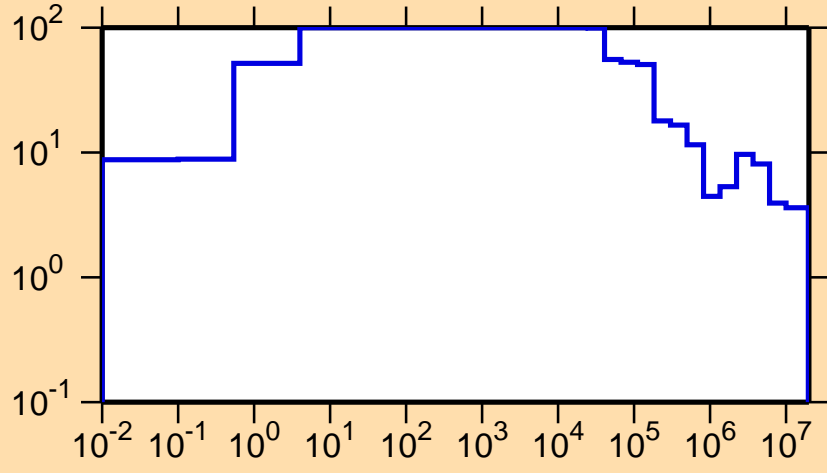
\Delta\sigma/\sigma vs. E for ^{134}\text{Pm}(n,el.)
