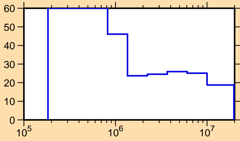
\Delta\sigma/\sigma vs. E for ^{134}\text{Pm}(n,n_1)
