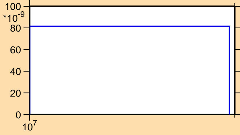
\sigma vs. E for ^{134}\text{Pm}(n,pt)
