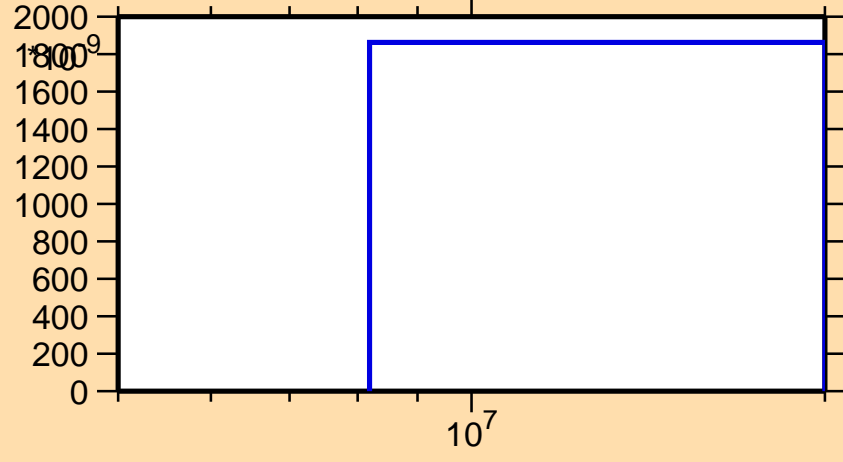
\sigma vs. E for ^{134}\text{Pm}(n,pd)
