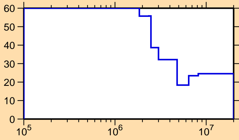
\Delta\sigma/\sigma vs. E for ^{134}\text{Pm}(n,ncont.)
