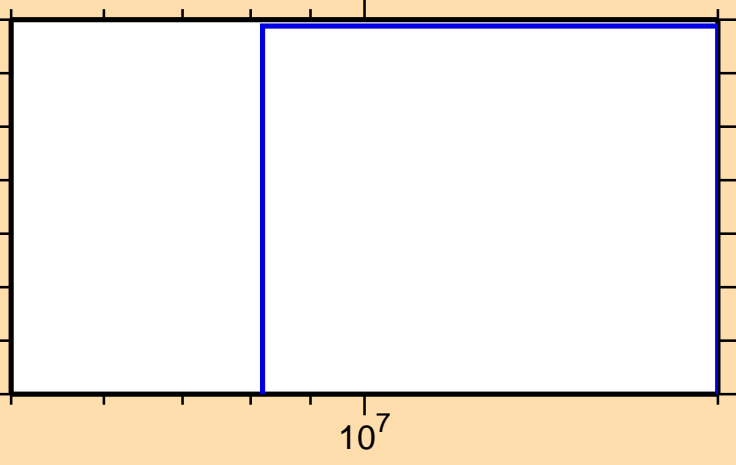
\sigma vs. E for ^{134}\text{Pm}(n,pt)
