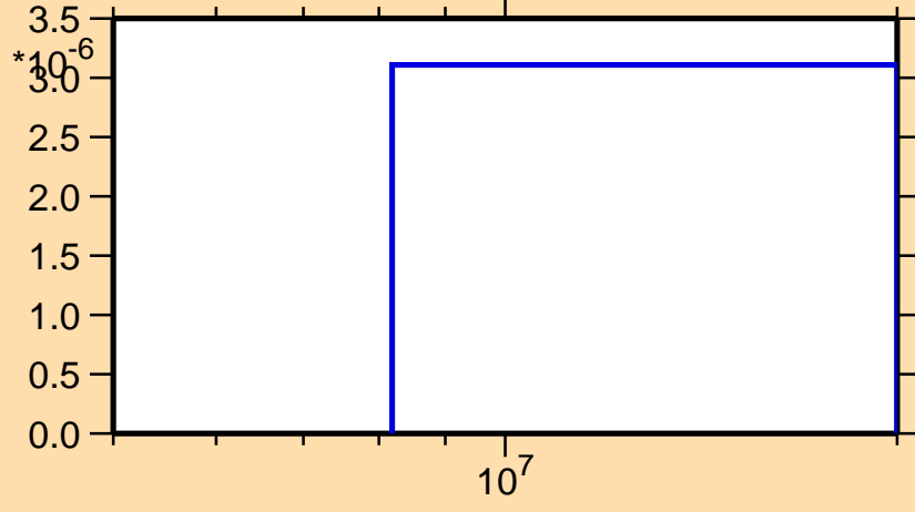
\sigma vs. E for ^{134}\text{Pm}(n,nd)
