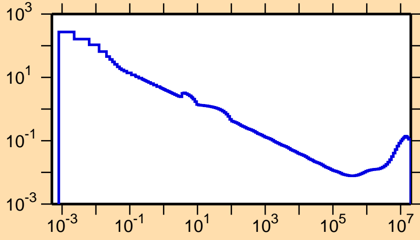
\sigma vs. E for ^{134}\text{Pm}(n,\alpha)
