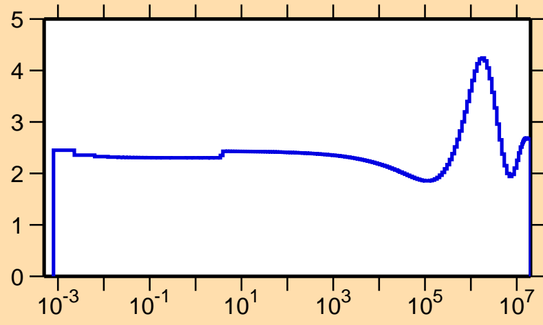
\sigma vs. E for ^{134}\text{Pm}(n,\text{el.})
