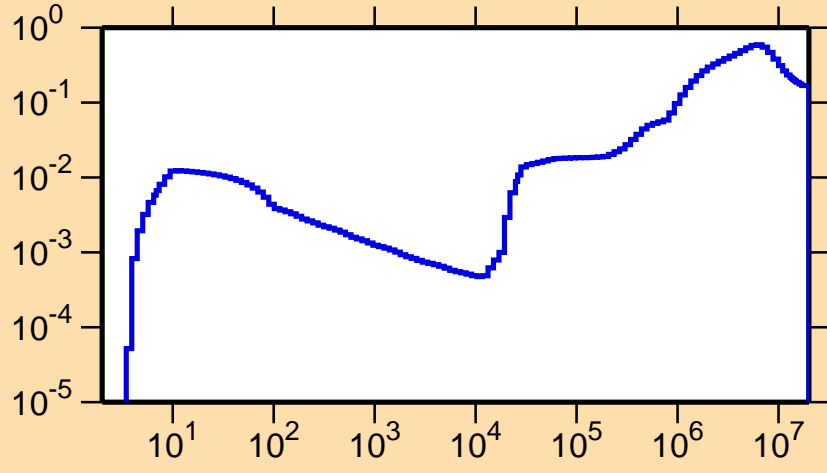
\sigma vs. E for ^{134}\text{Pm}(n,\text{inel.})
