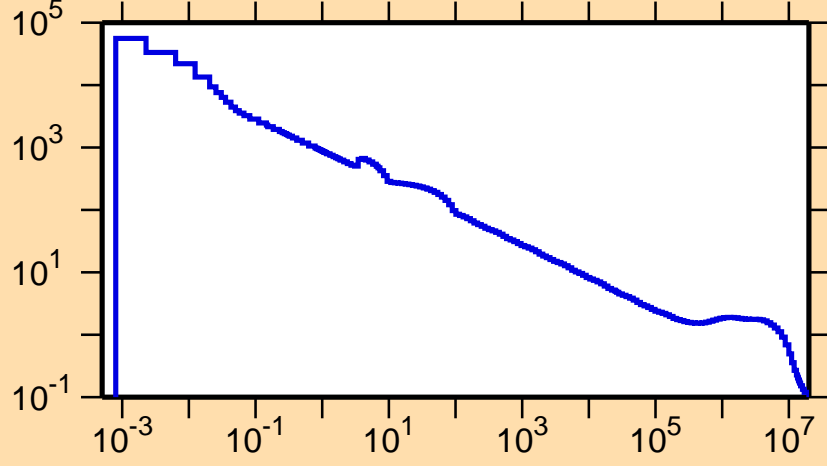
\sigma vs. E for ^{134}\text{Pm}(n,p)
