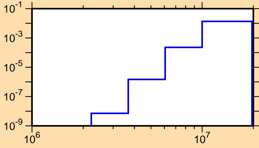
\sigma vs. E for ^{135}\text{Pm}(n,d)
