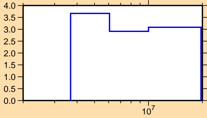
\Delta\sigma/\sigma vs. E for ^{135}\text{Pm}(n,n\text{onel.})
