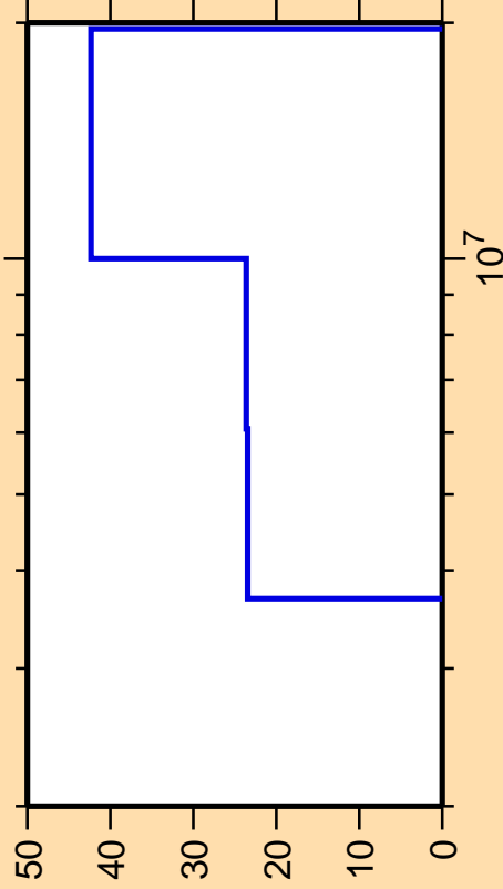
\Delta\sigma/\sigma vs. E for ^{135}\text{Pm}(n,n\text{cont.})
