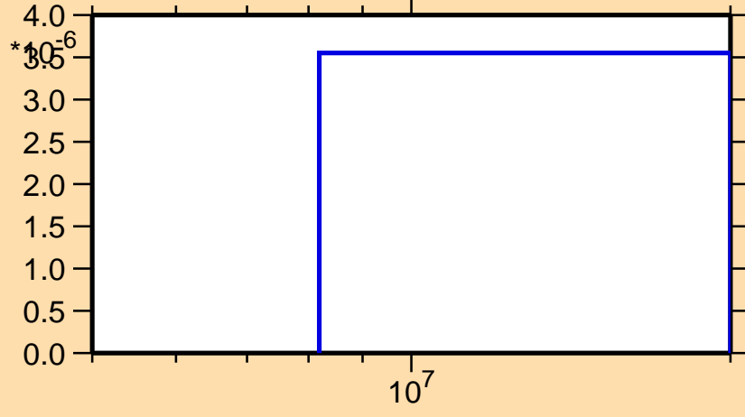
\sigma vs. E for ^{135}\text{Pm}(n,\text{pd})
