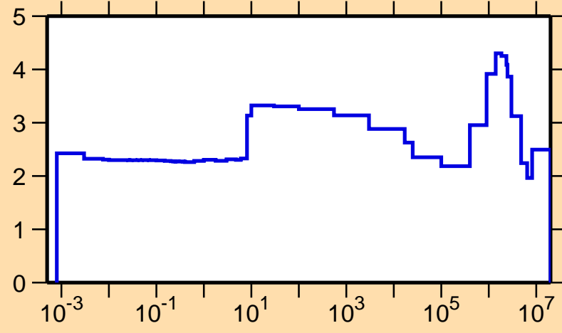
\sigma vs. E for ^{135}\text{Pm}(n,\text{el.})
