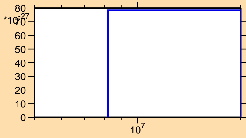
\sigma vs. E for ^{135}\text{Pm} (mt 11)
