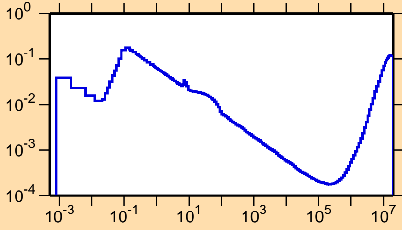
\sigma vs. E for ^{135}\text{Pm}(n,\alpha)
