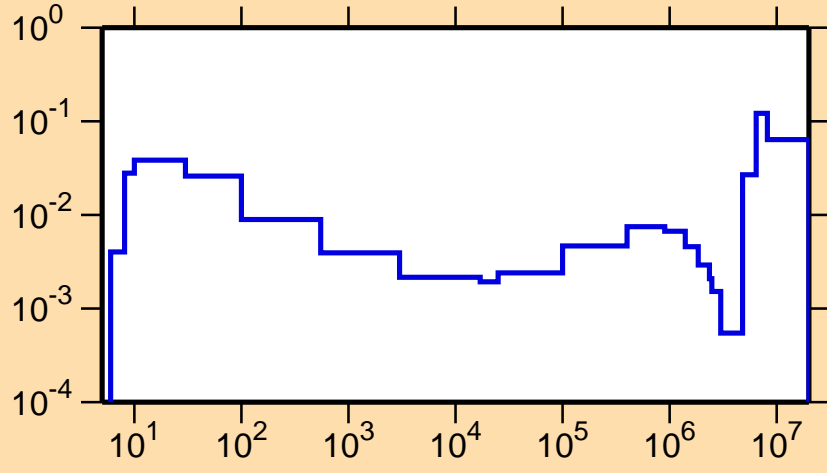
\sigma vs. E for ^{135}\text{Pm}(n,\text{inel.})
