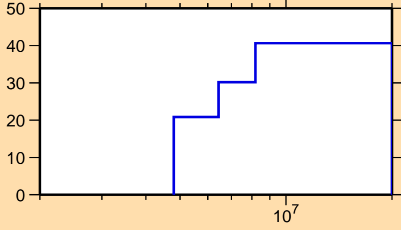
\Delta\sigma/\sigma vs. E for ^{135}\text{Pm}(n,n\text{cont.})
