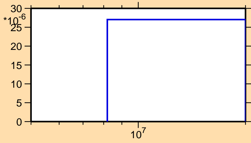
\sigma vs. E for ^{135}\text{Pm}(n,2np)
