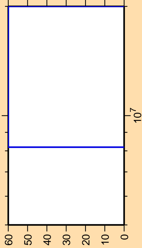
\Delta\sigma/\sigma vs. E for ^{135}\text{Pm}(n,pd)
