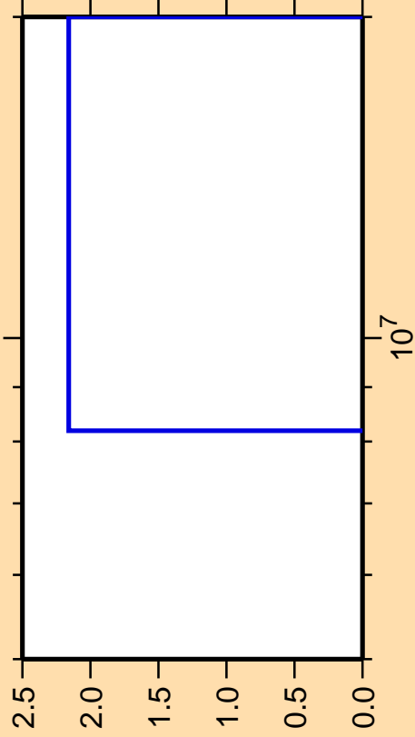
\Delta\sigma/\sigma vs. E for ^{135}\text{Pm} (mt 34)
