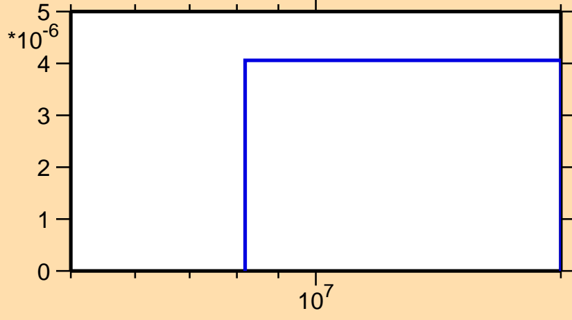
\sigma vs. E for ^{135}\text{Pm}(n,pd)
