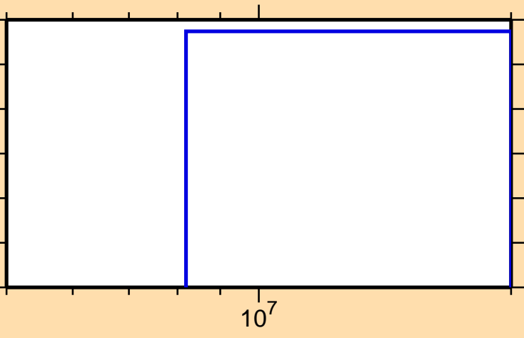
\sigma vs. E for ^{135}\text{Pm} (mt 34)
