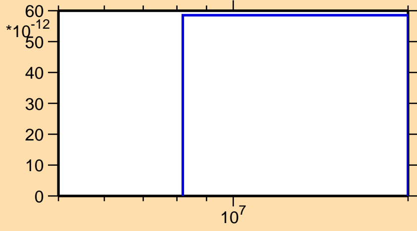
\sigma vs. E for ^{135}\text{Pm}(n,\text{pt})
