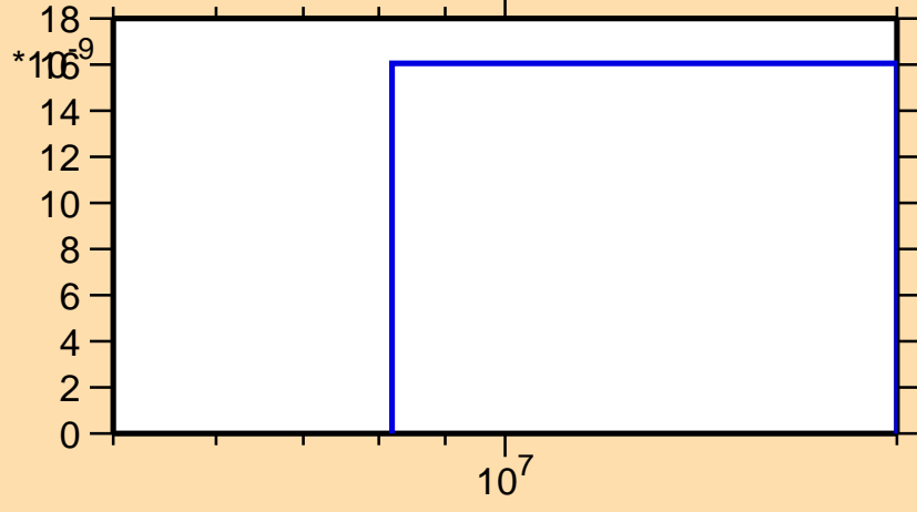
\sigma vs. E for ^{135}\text{Pm}(\text{mt117})
