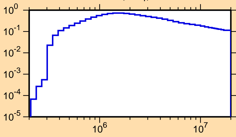
\sigma vs. E for ^{136}\text{Pm}(n,n_1)
