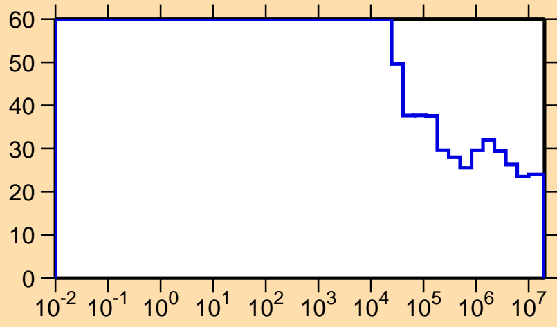
\Delta\sigma/\sigma vs. E for ^{136}\text{Pm}(n,p)
