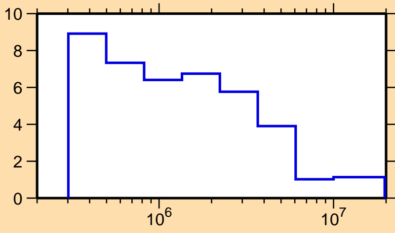
\Delta\sigma/\sigma vs. E for ^{136}\text{Pm}(n,\text{tot.})
