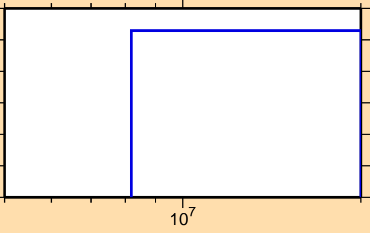
\sigma vs. E for ^{136}\text{Pm}(n,2np)
