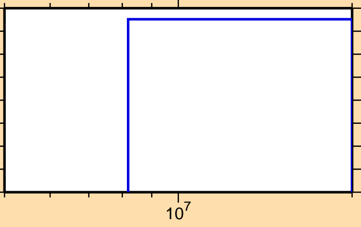
\sigma vs. E for ^{136}\text{Pm} (mt 45)
