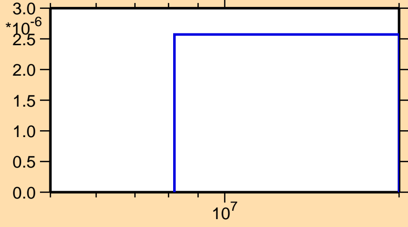
\sigma vs. E for ^{136}\text{Pm}(n,\text{nd})
