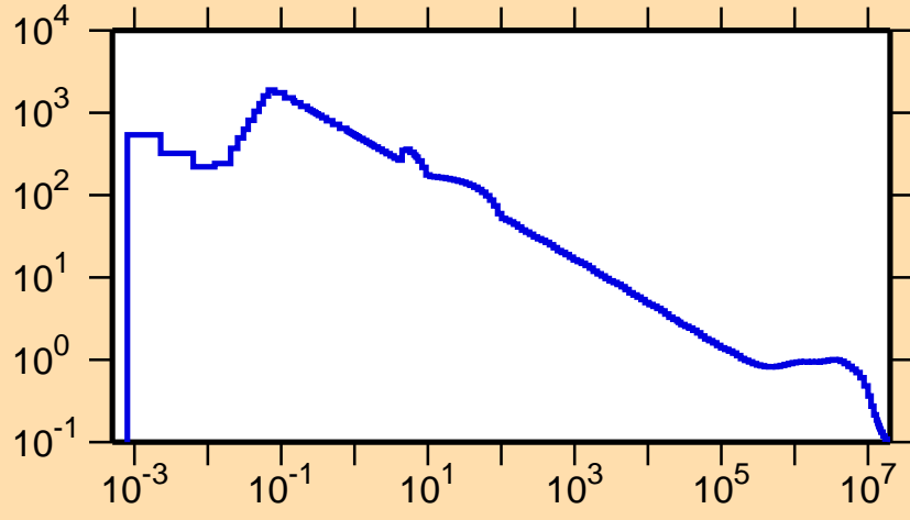
\sigma vs. E for ^{136}\text{Pm}(n,p)
