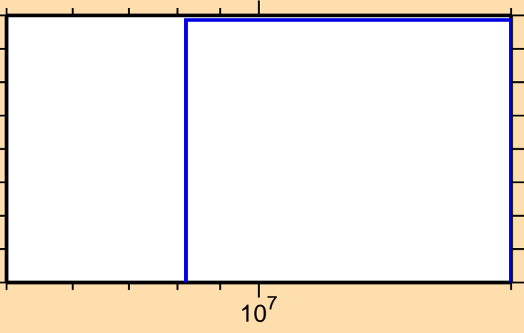
\sigma vs. E for ^{136}\text{Pm}(n,2np)
